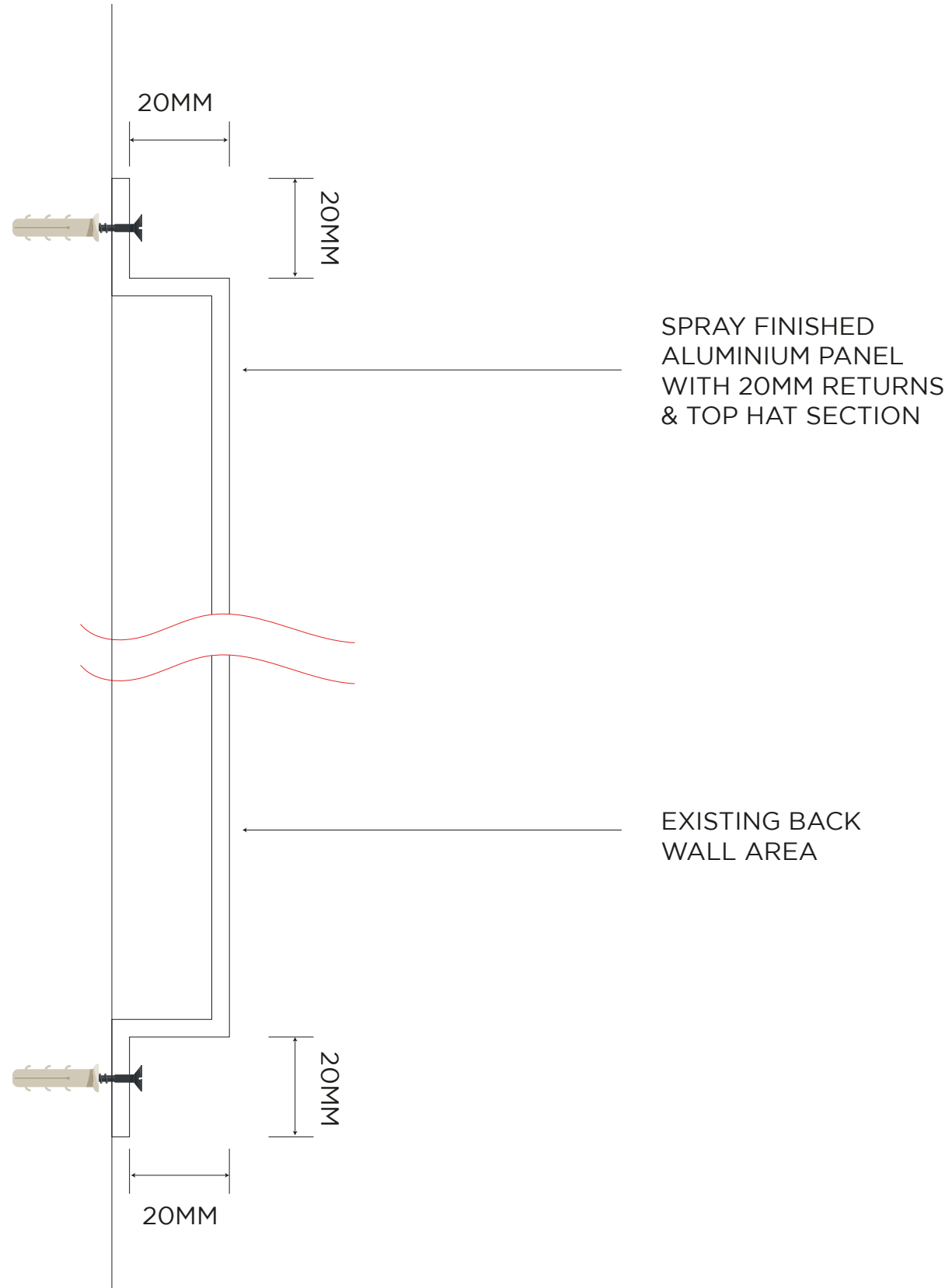
FIXING DETAIL - 1:10
