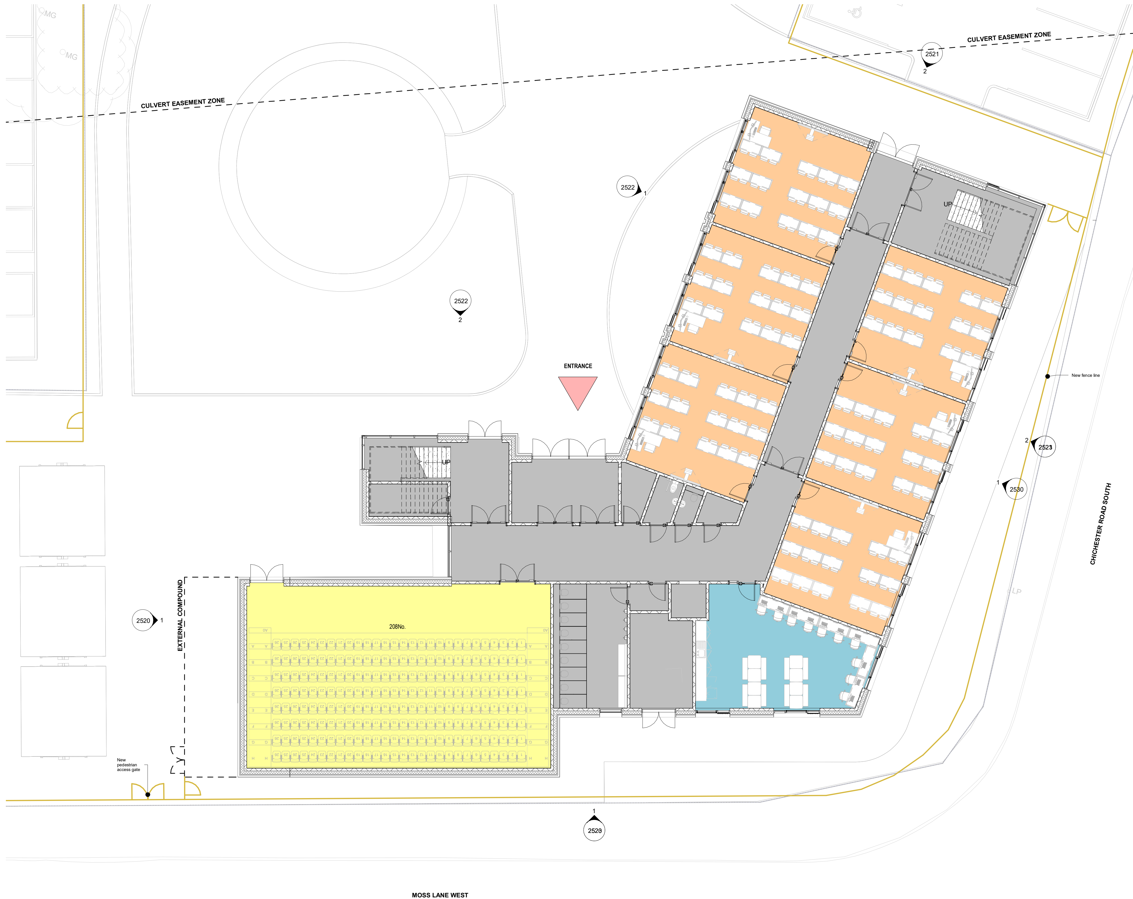
1 Ground Floor Proposed Plan 1 : 100 Ref Sheet: 2520
