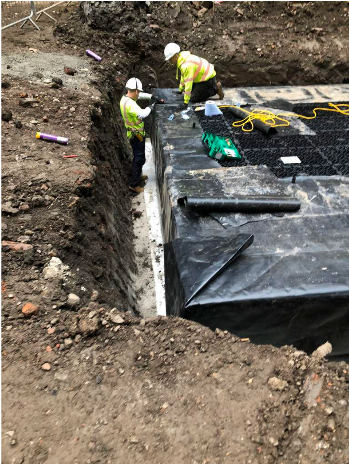
Surface water retention tank
