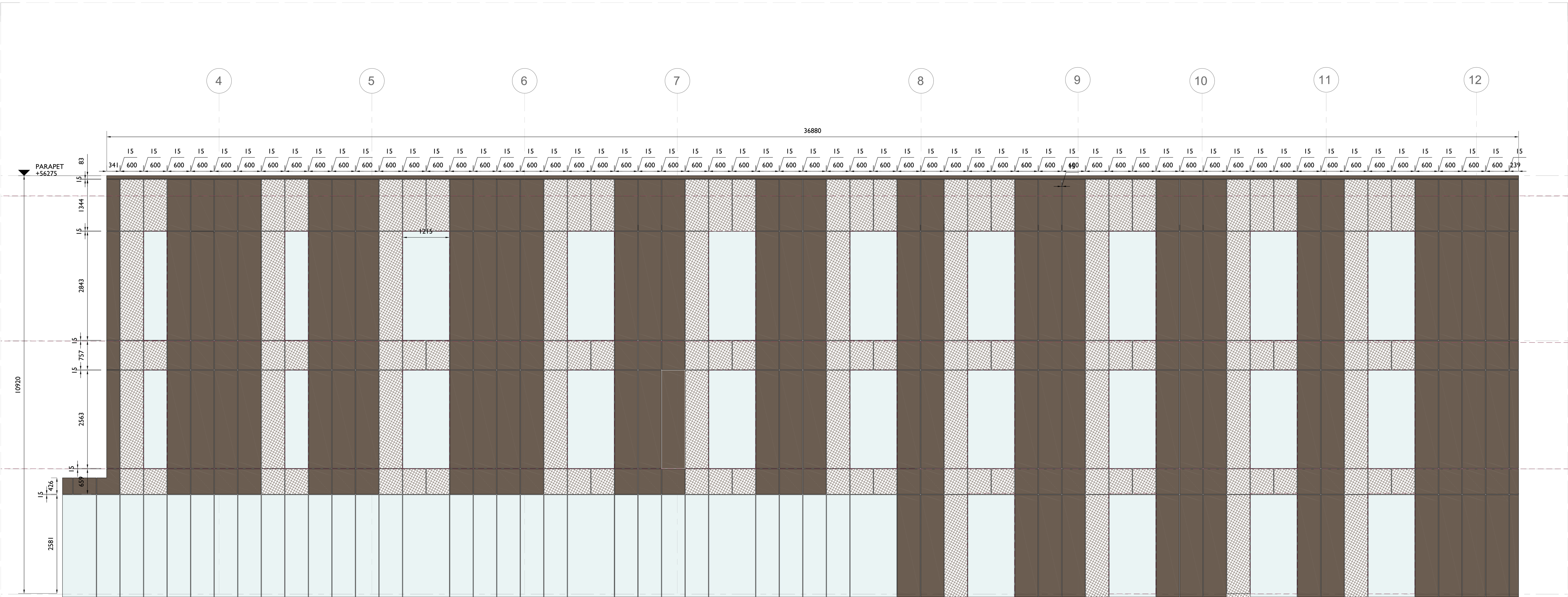
1 4200 Elevation 3 Setting Out 1:50
