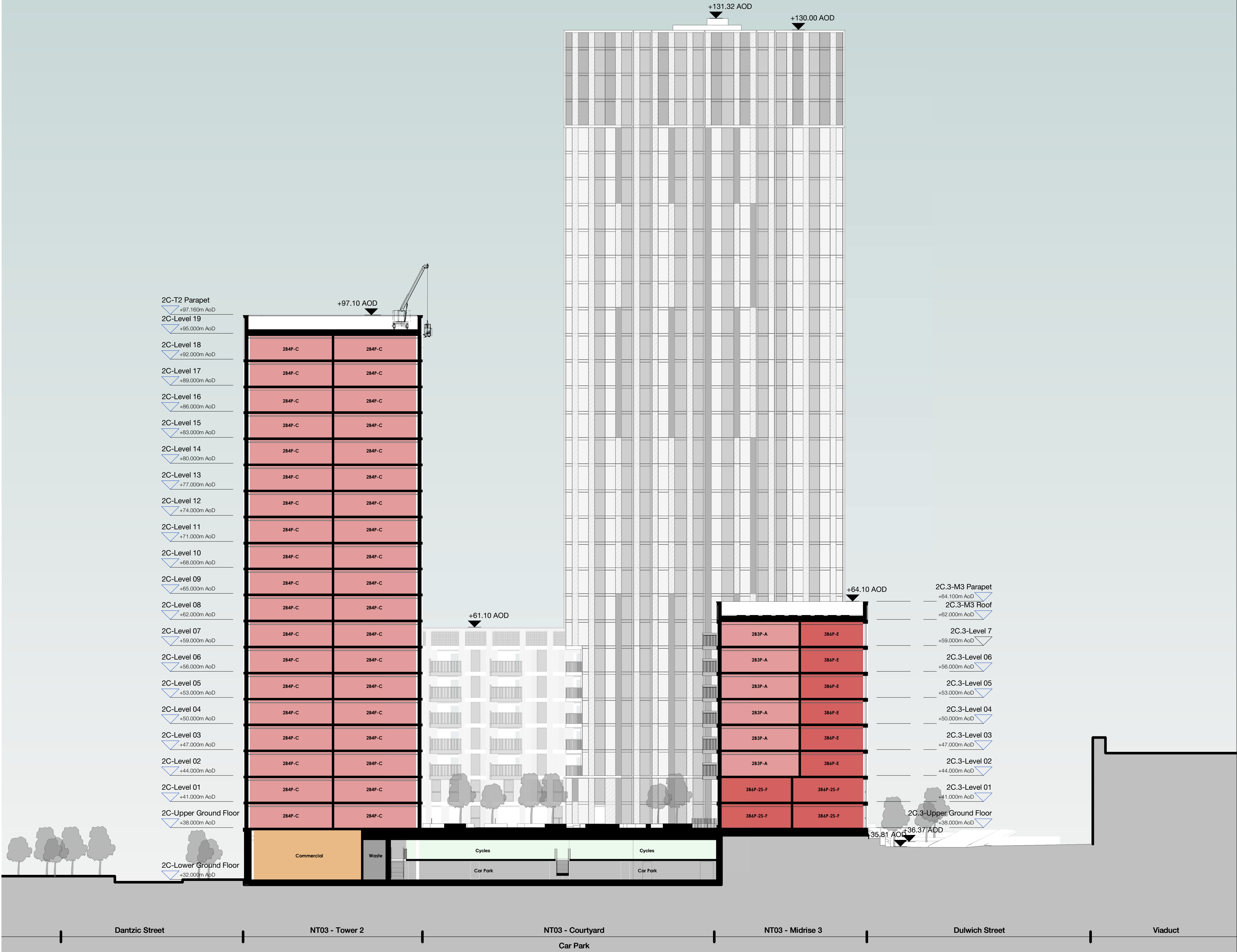
Planning-NT03 - Proposed Section B-B 1 : 250
