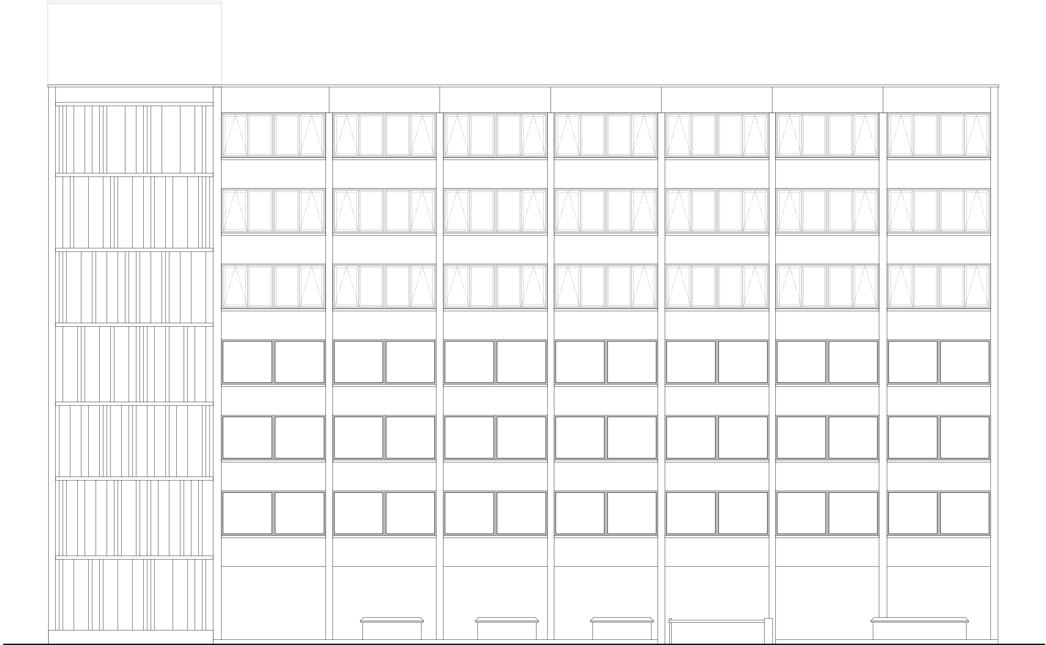
1 ELEVATION C (MAJOR ST) Scale: 1:100
