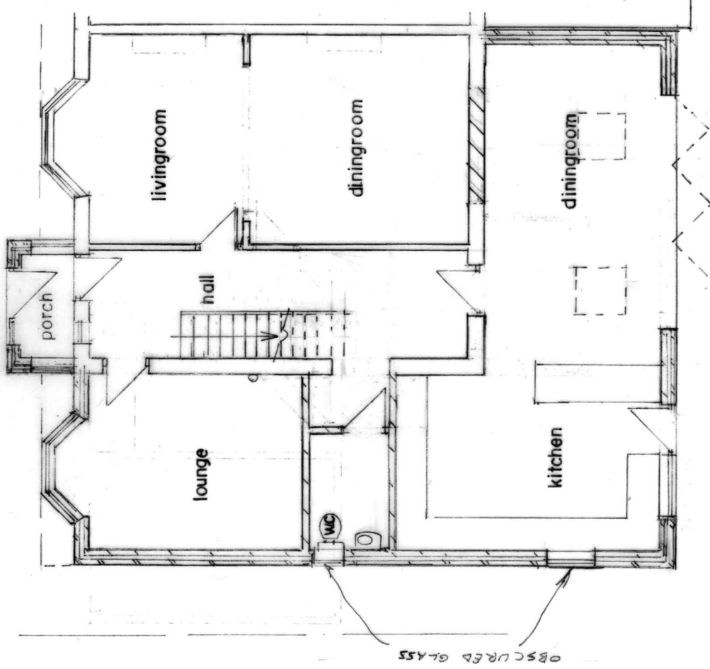
GROUND FLOOR PLAN (PROPOSED)
