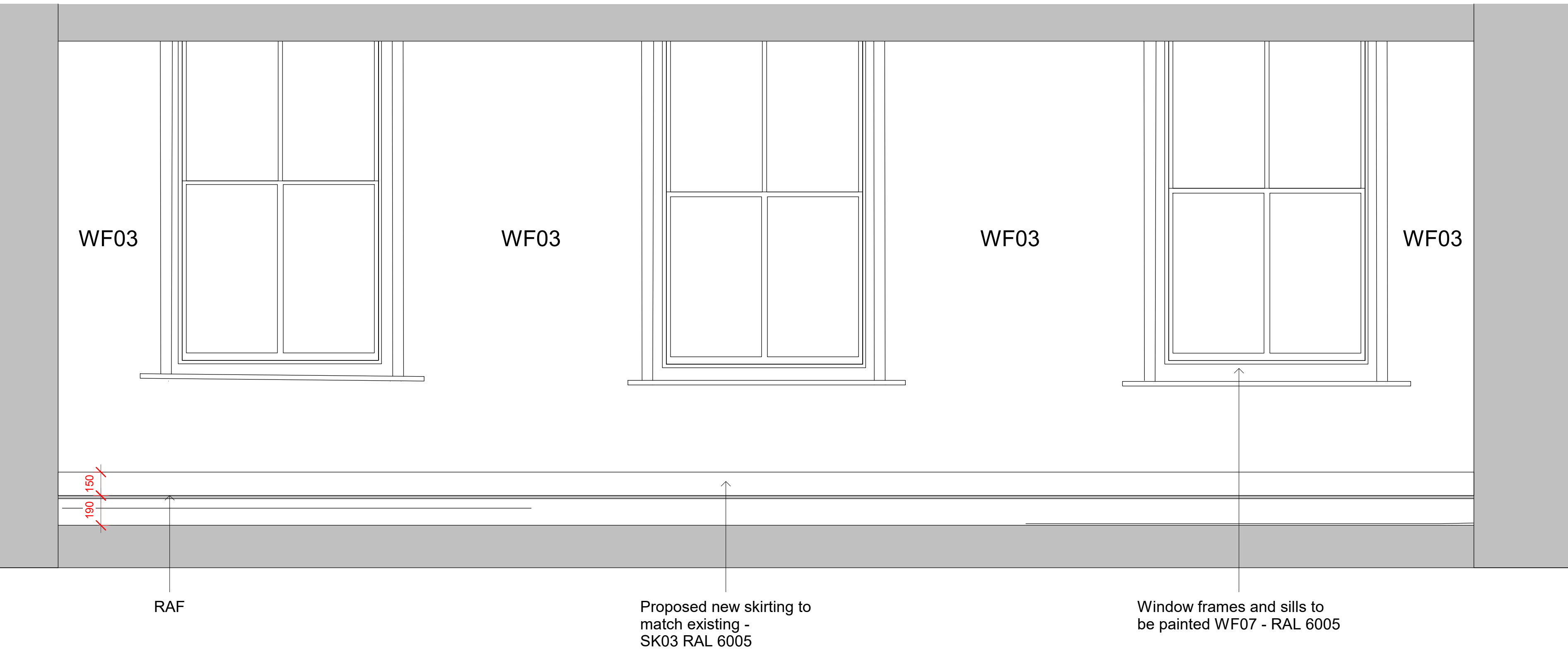
2FL - Elevation 8 1 : 20
