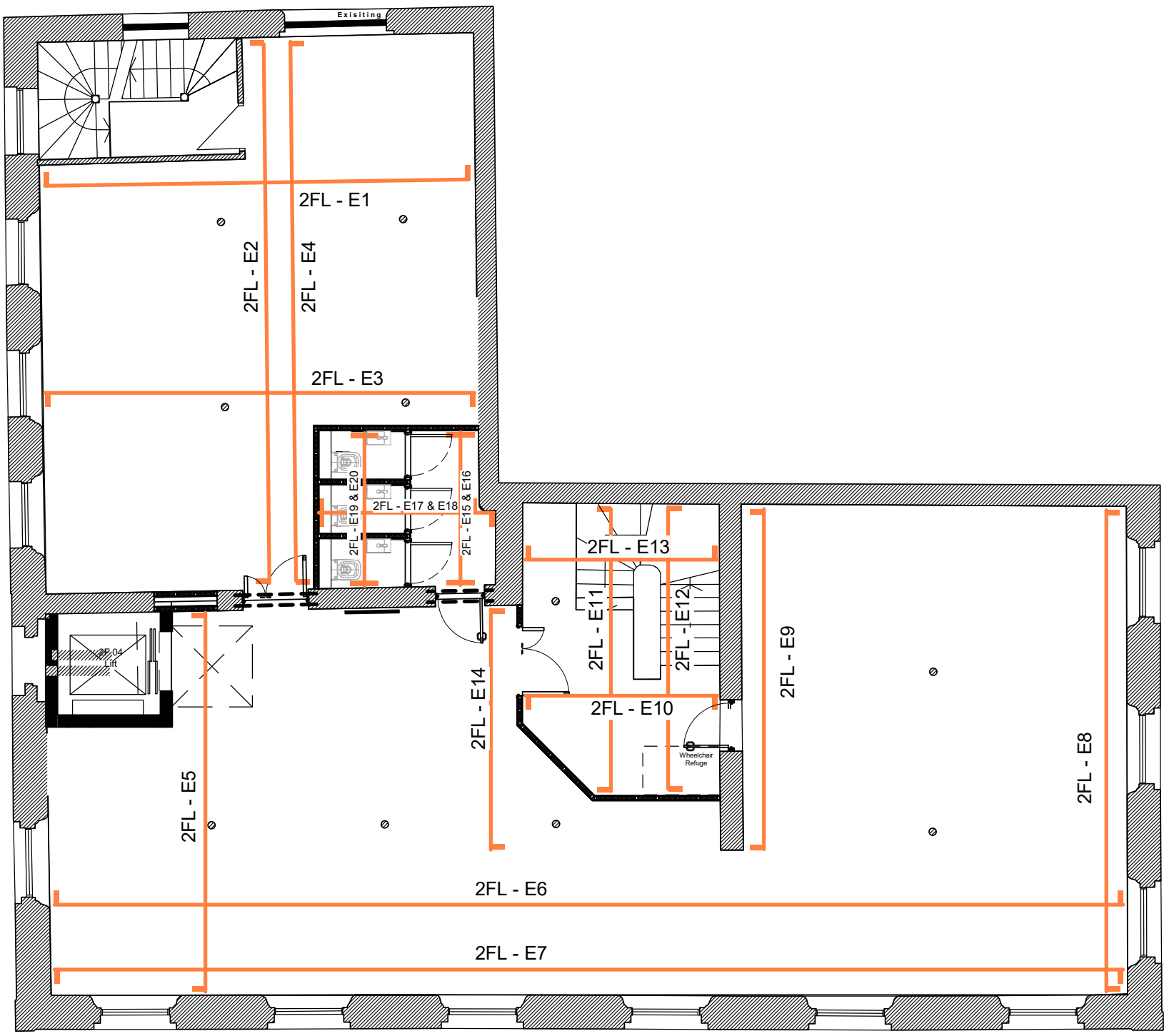
2FL Proposed Internal Elevation Layout_01 1 : 100
