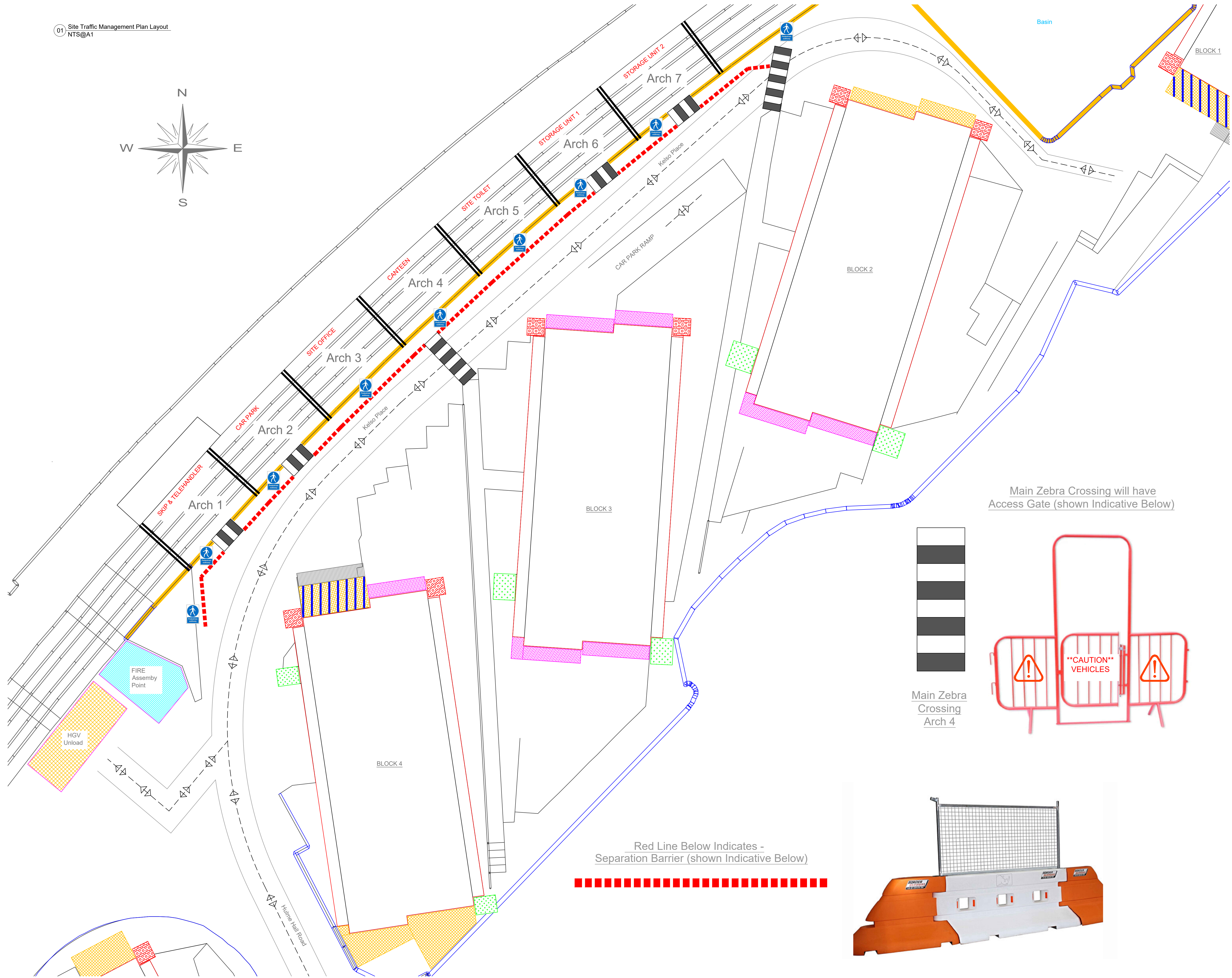
Access/Resident Walkway
