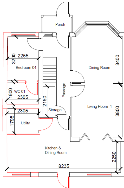
Ground Floor Plan as Proposed
