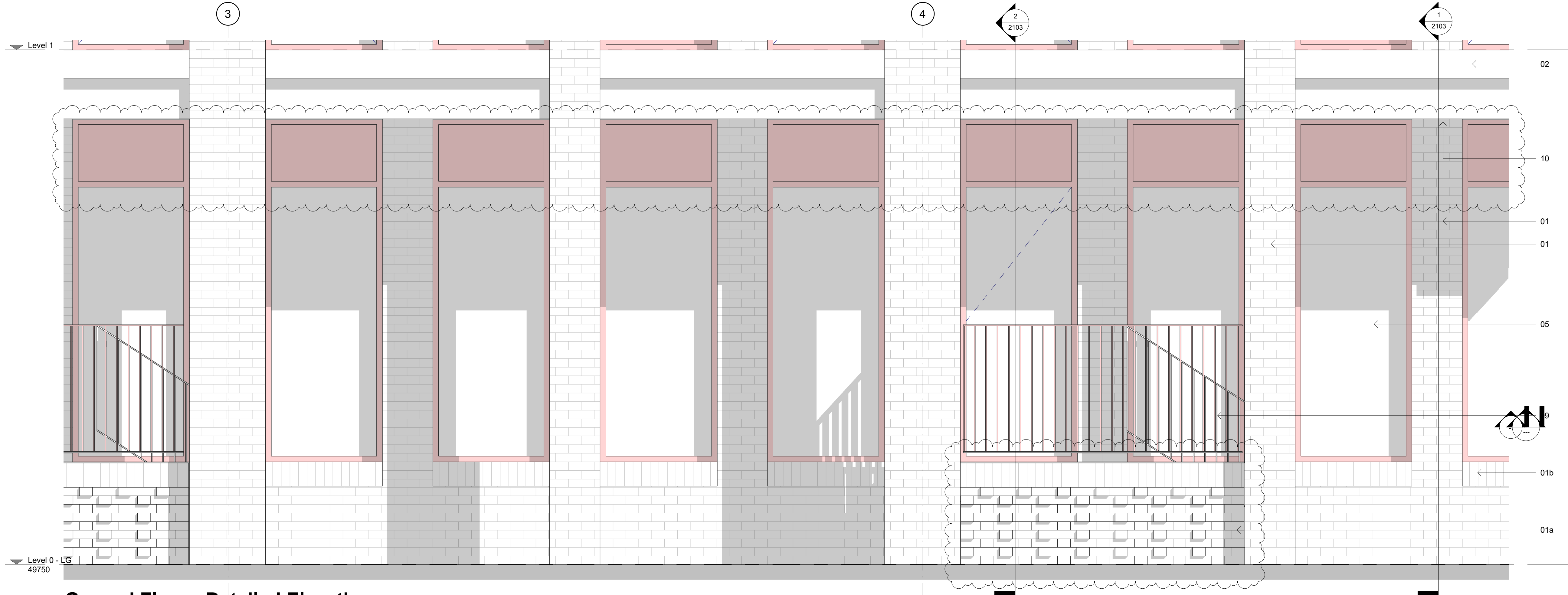
Ground Floor - Detailed Elevation 1 : 20
