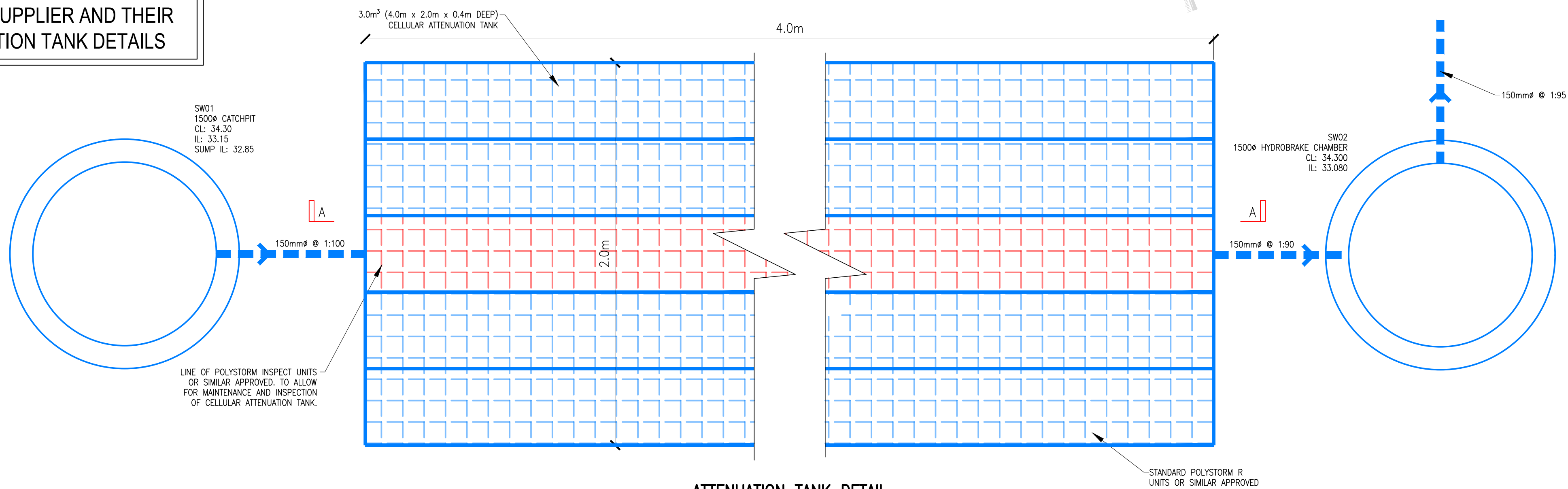
ATTENUATION TANK DETAIL
