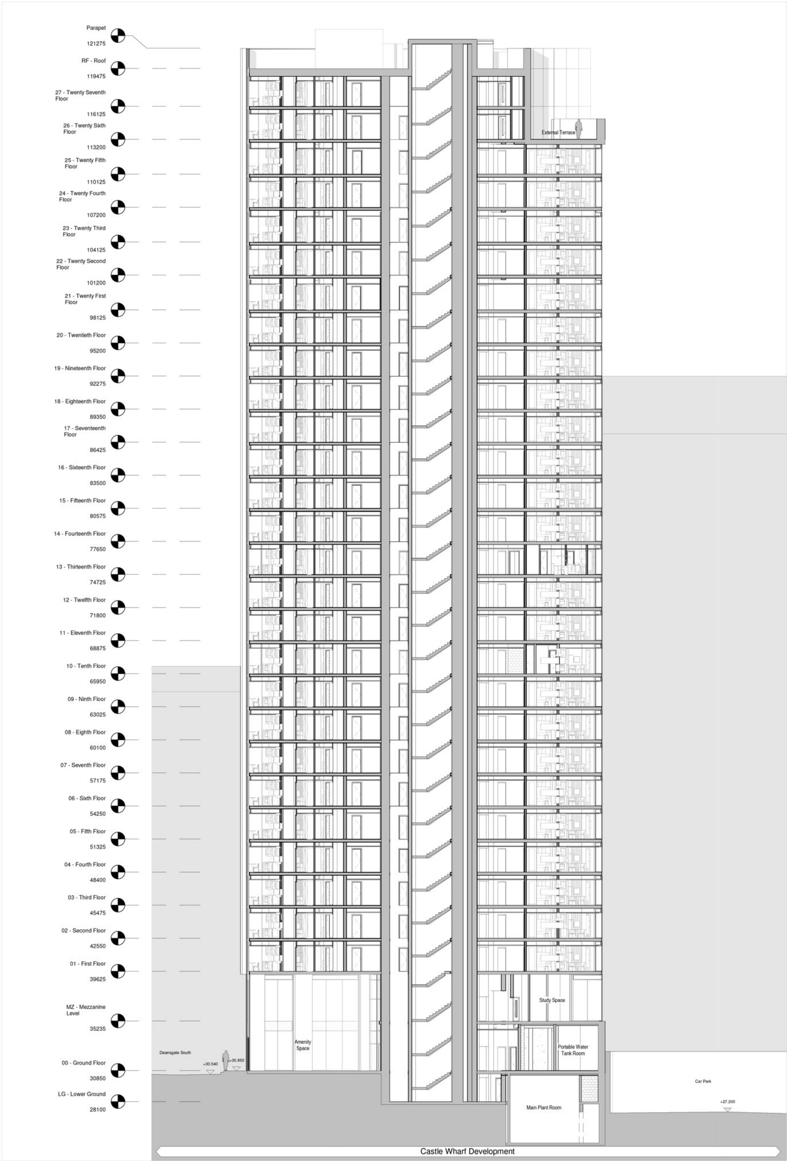
01 Section B-B 1:200
