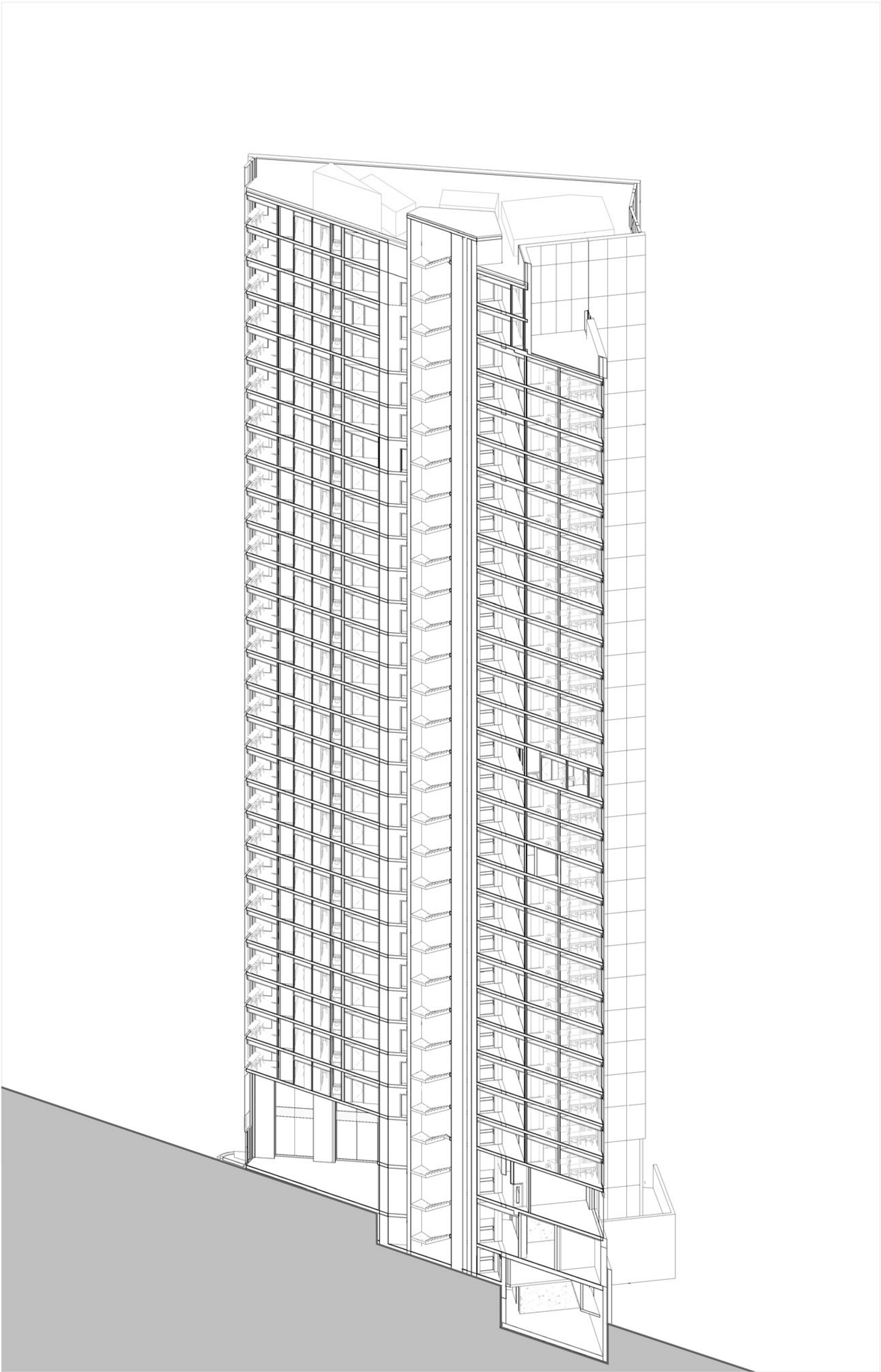
02 1:200 - 3D View - Section - B-B
