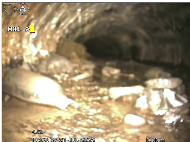
Photo: 4_4a, 00:00:00 0.2m, Debris silt, 25 % cross-sectional area loss, Start
