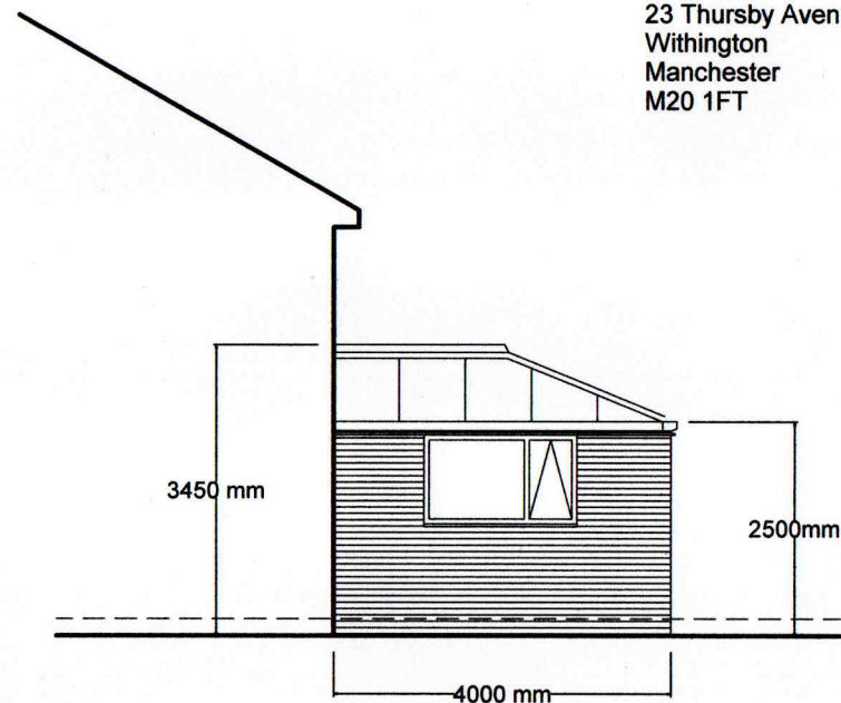
Proposed Side Section Elevation 1:100
