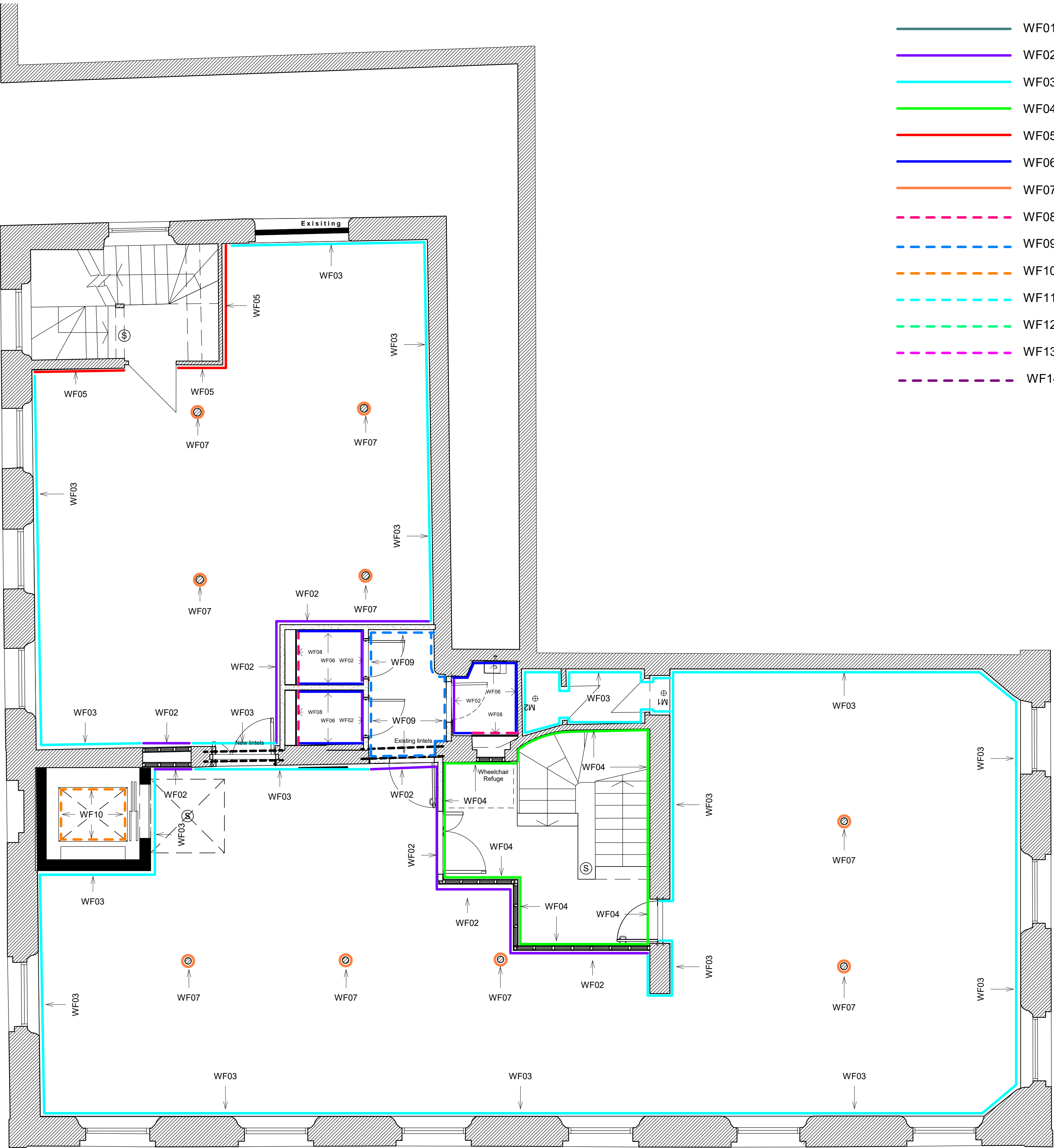
1FL Proposed Wall Finishes 1 : 50
