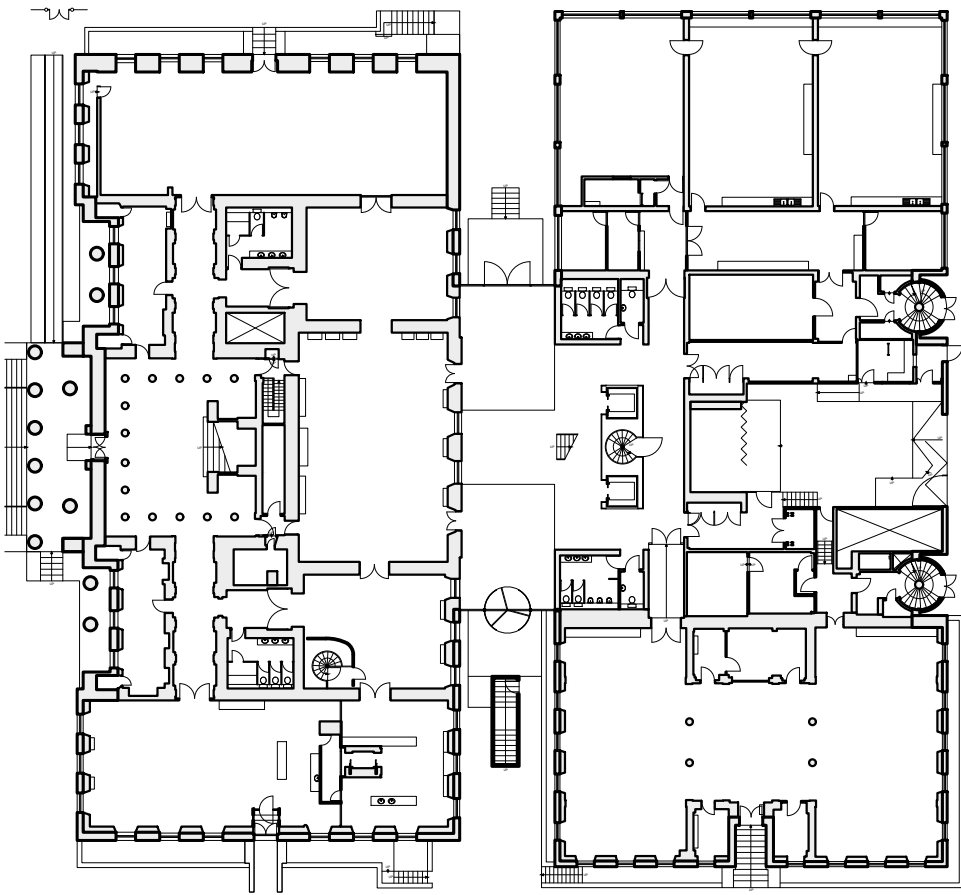
KEY PLAN
