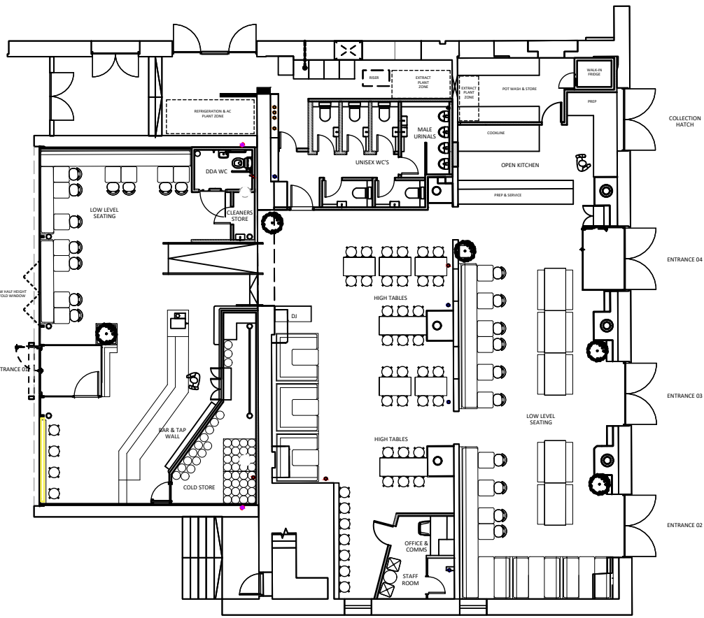
01 132 GROUND FLOOR PLAN AS PROPOSED SCALE - 1:200 @ A1 PLAN
