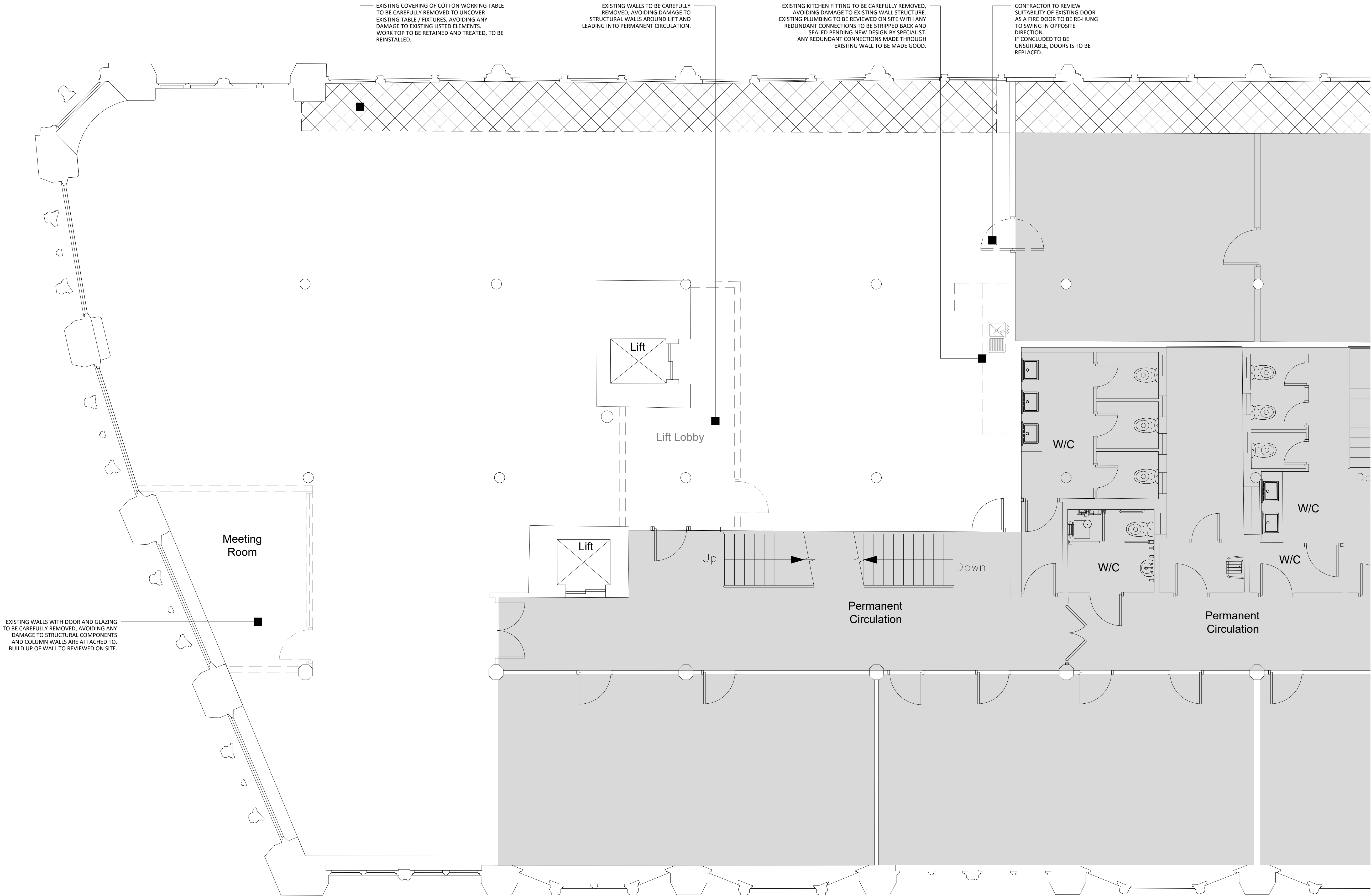
01 063 PROPOSED THIRD FLOOR SUITE BWIC PLAN SCALE - 1:50 @ A1 AS PROPOSED
