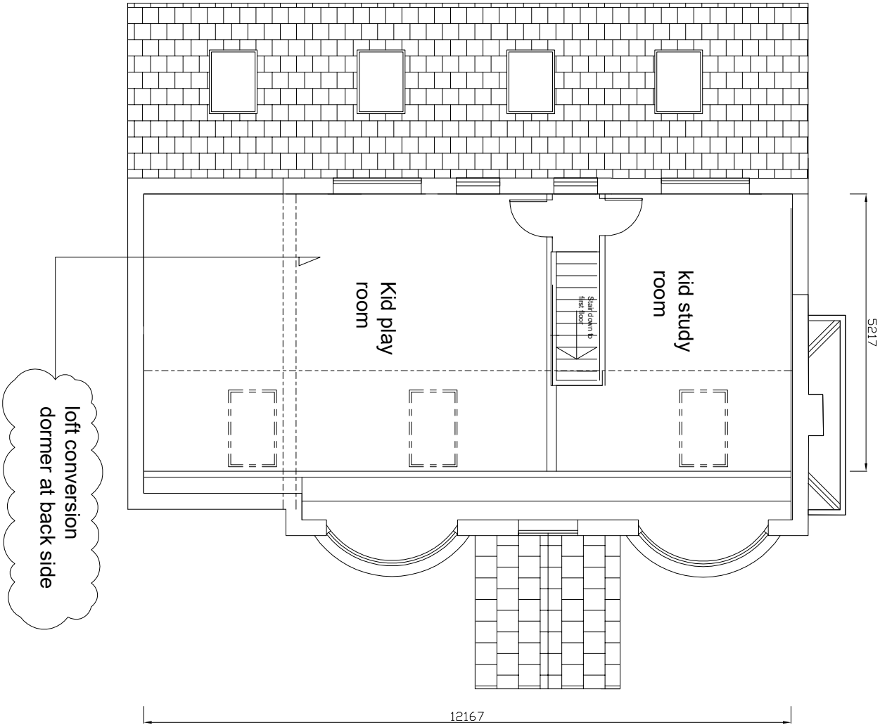
- LAYOUT FLOOR PLAN PROPOSED PLAN Loft 1 : 100 ( IN A3)
