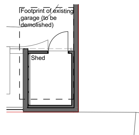
5 GF-Ground Floor 1:100
