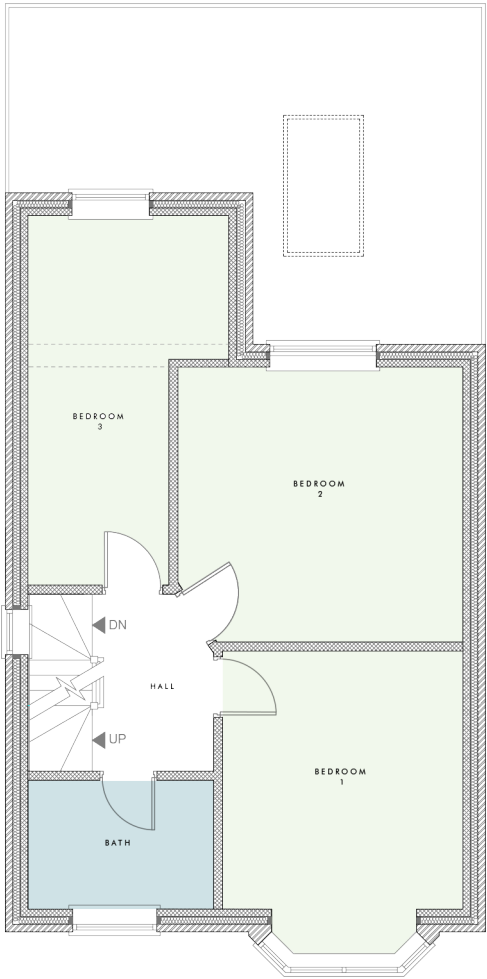
PROPOSED FIRST FLOOR PLAN 1:100 @ A3
