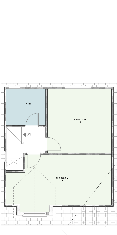
PROPOSED LOFT PLAN 1:100 @ A3
