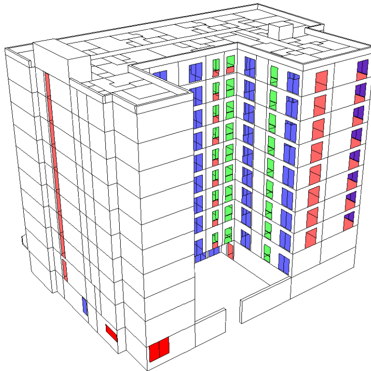
Figure 4. Showing opening types from East
