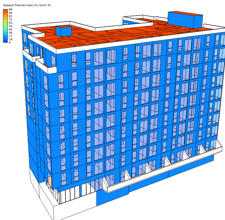
Figure 2. Thermal Mass Cm for Opaque Building Fabric
