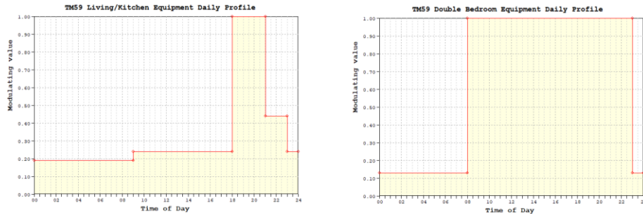
Figure 7. Kitchen/Living/Dining and Double Bedroom Modulating Profile for Equipment Gains
