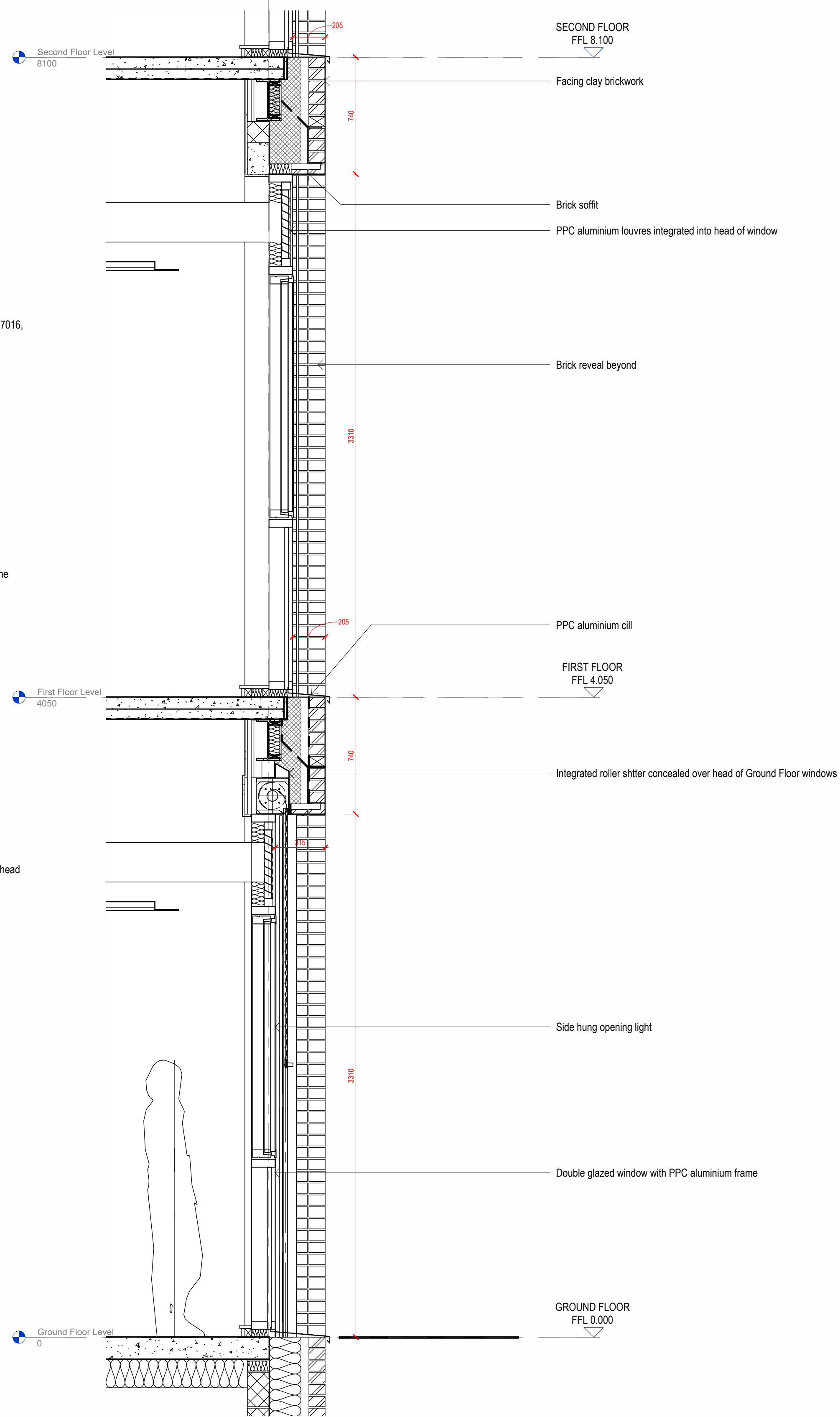
2 Chichester Road - Typical Bay Section 1:20 Ref Sheet: 2530
