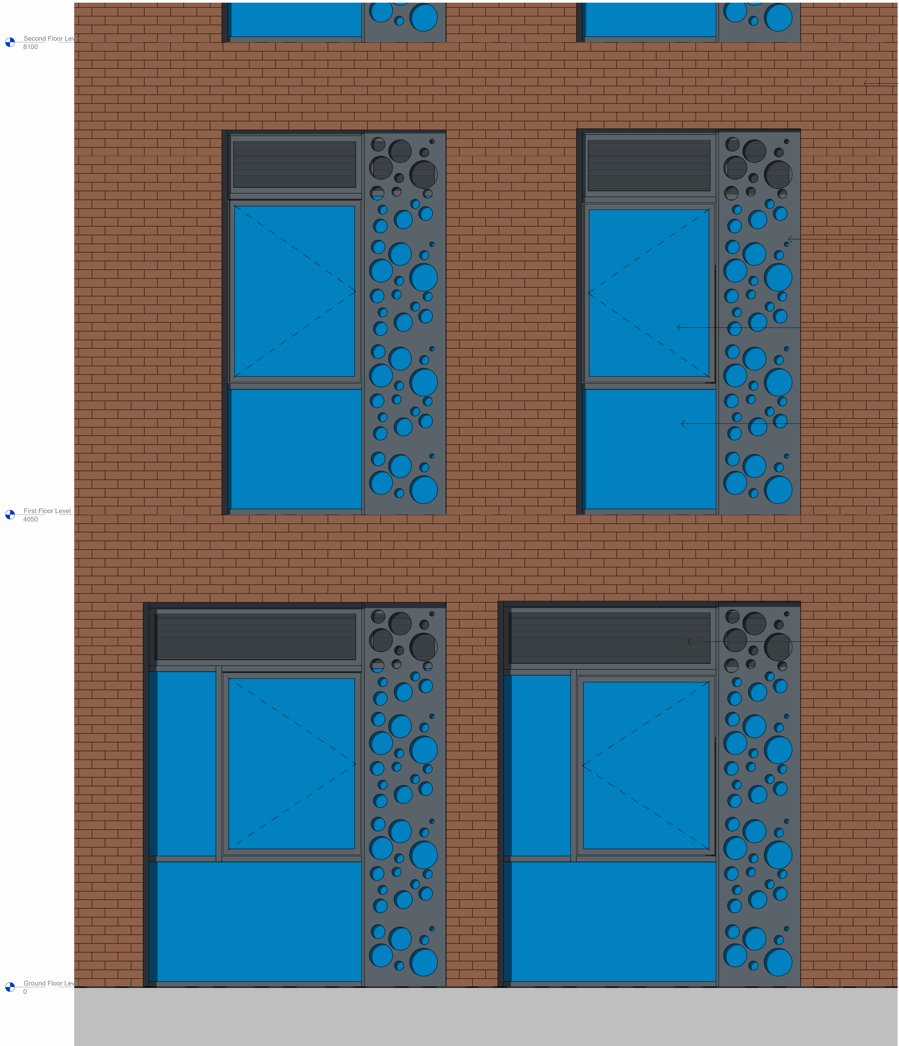
1 Chichester Road Elevation - Typical Bay 1:20 Ref Sheet: 0700
