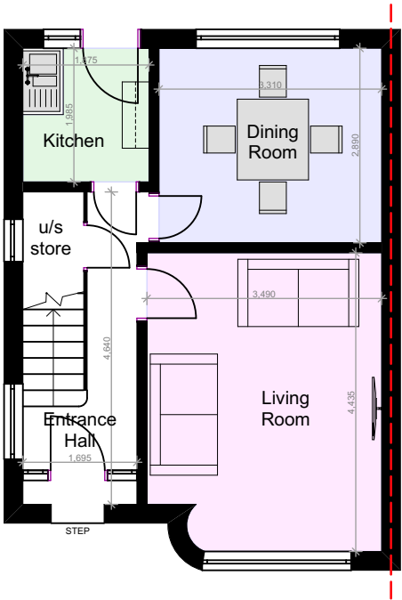
EXISTING GA GROUND FLOOR PLAN @ 1:100
