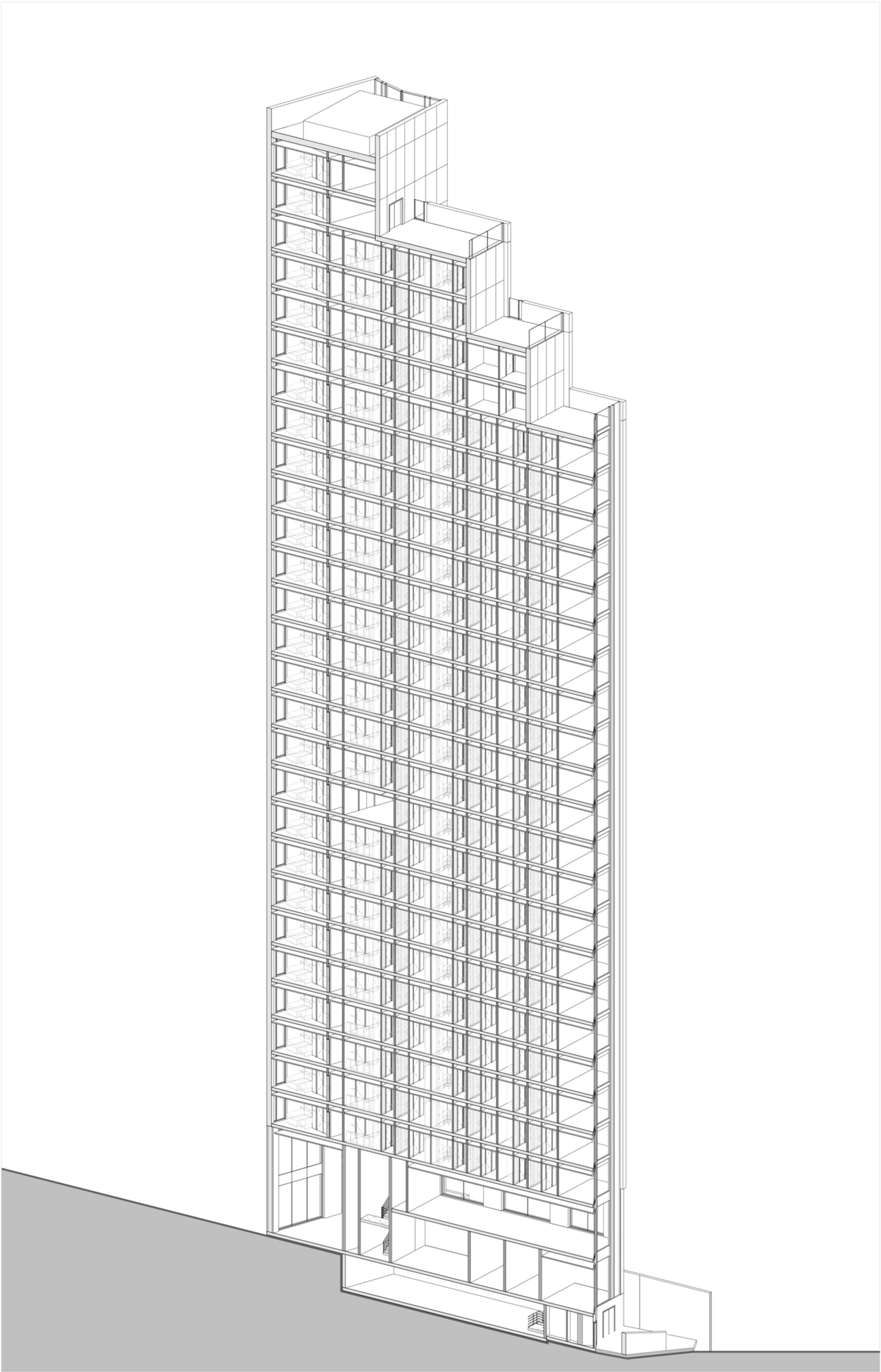
02 1.200 - 3D View - Section - C-C
