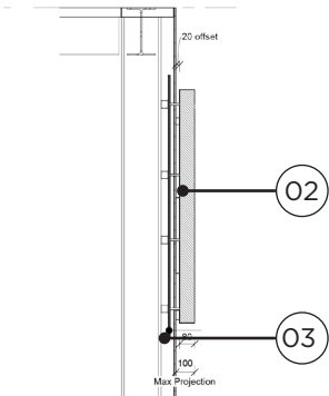
Type 01 - External Signage Section
