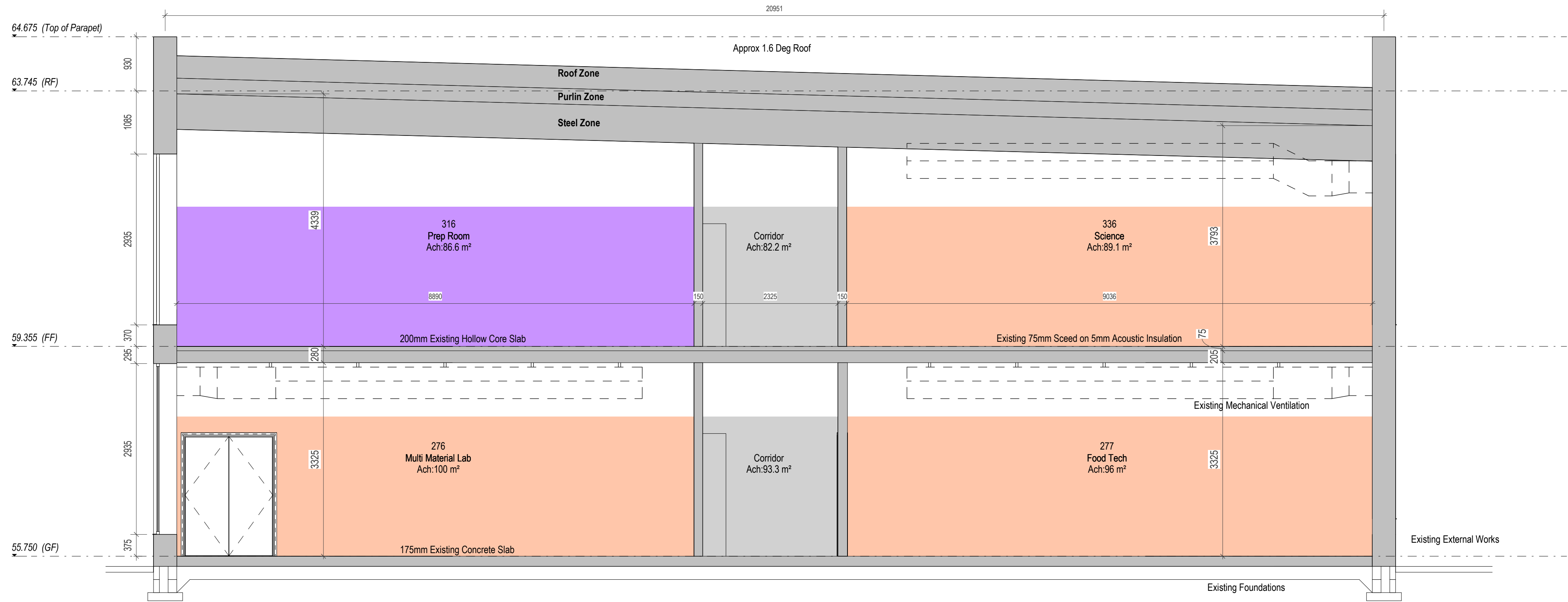
Existing Section 1 - 1
