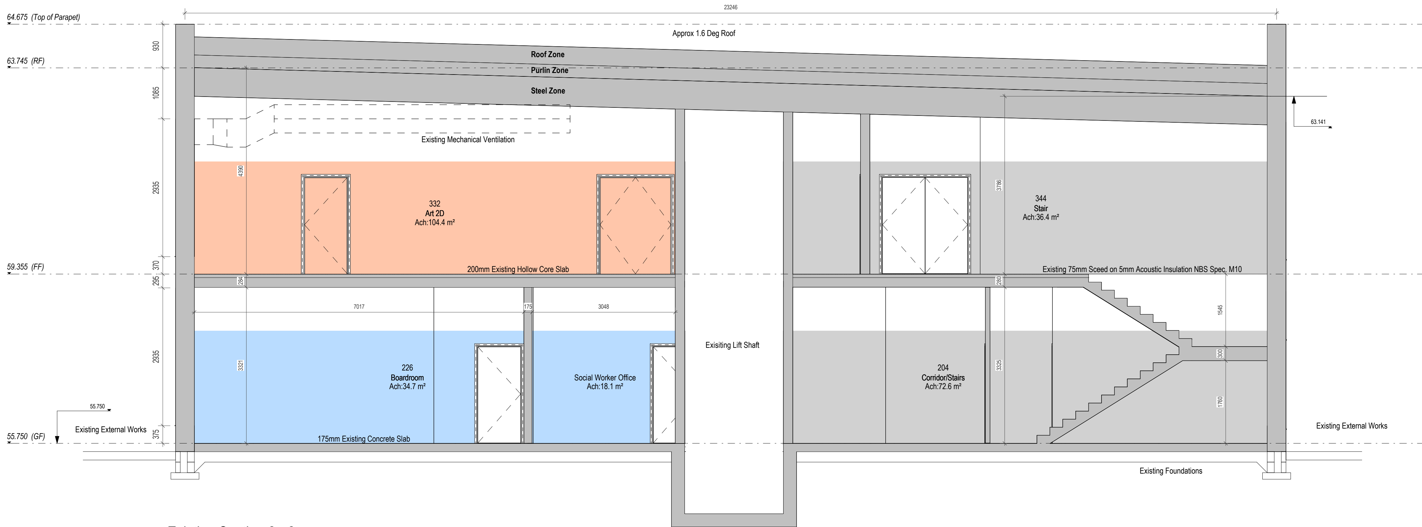
Existing Section 2 - 2
