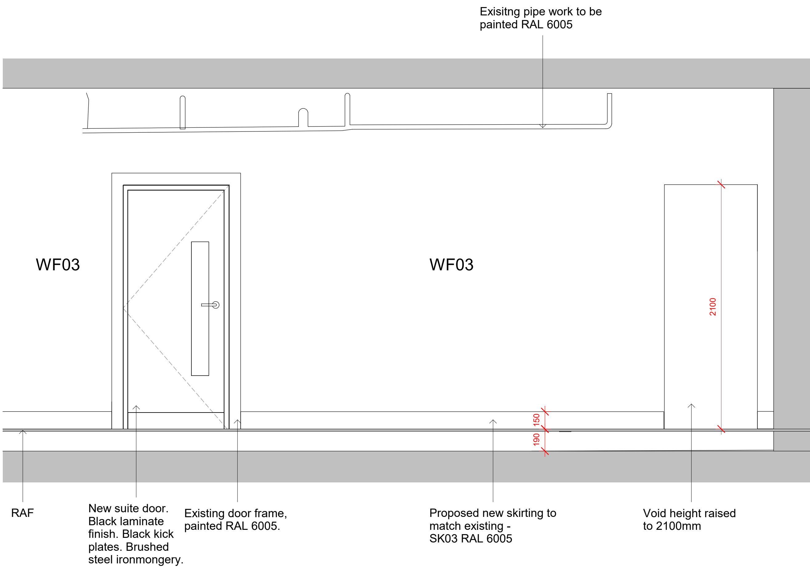
1FL - Elevation 9 1 : 20
