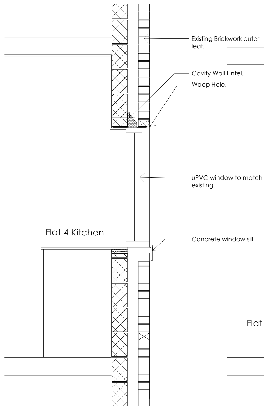
Window WS7 Detail 1:20
