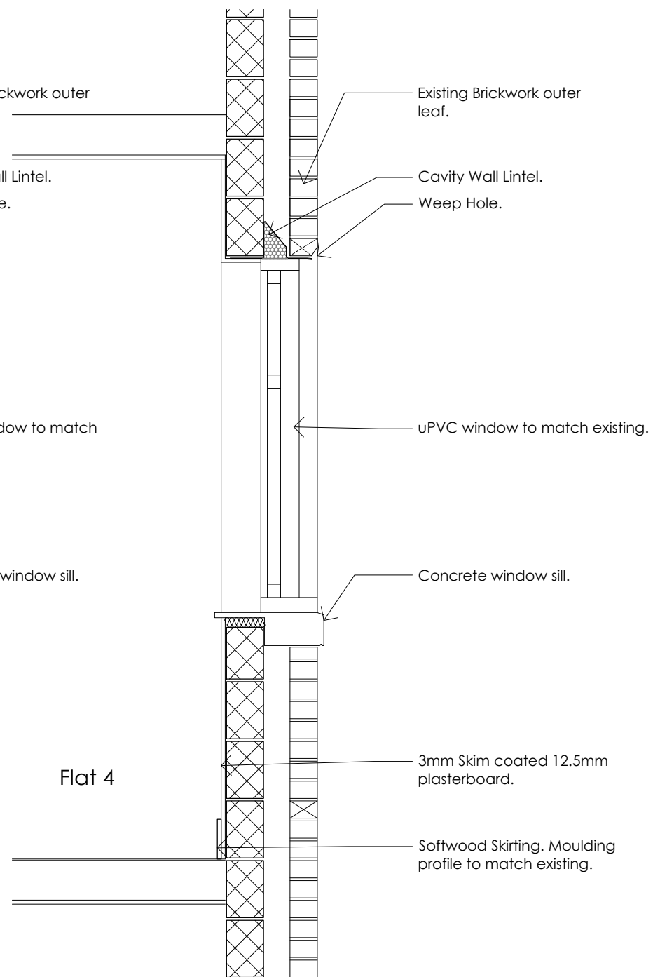
Window WS8 Detail 1:20
