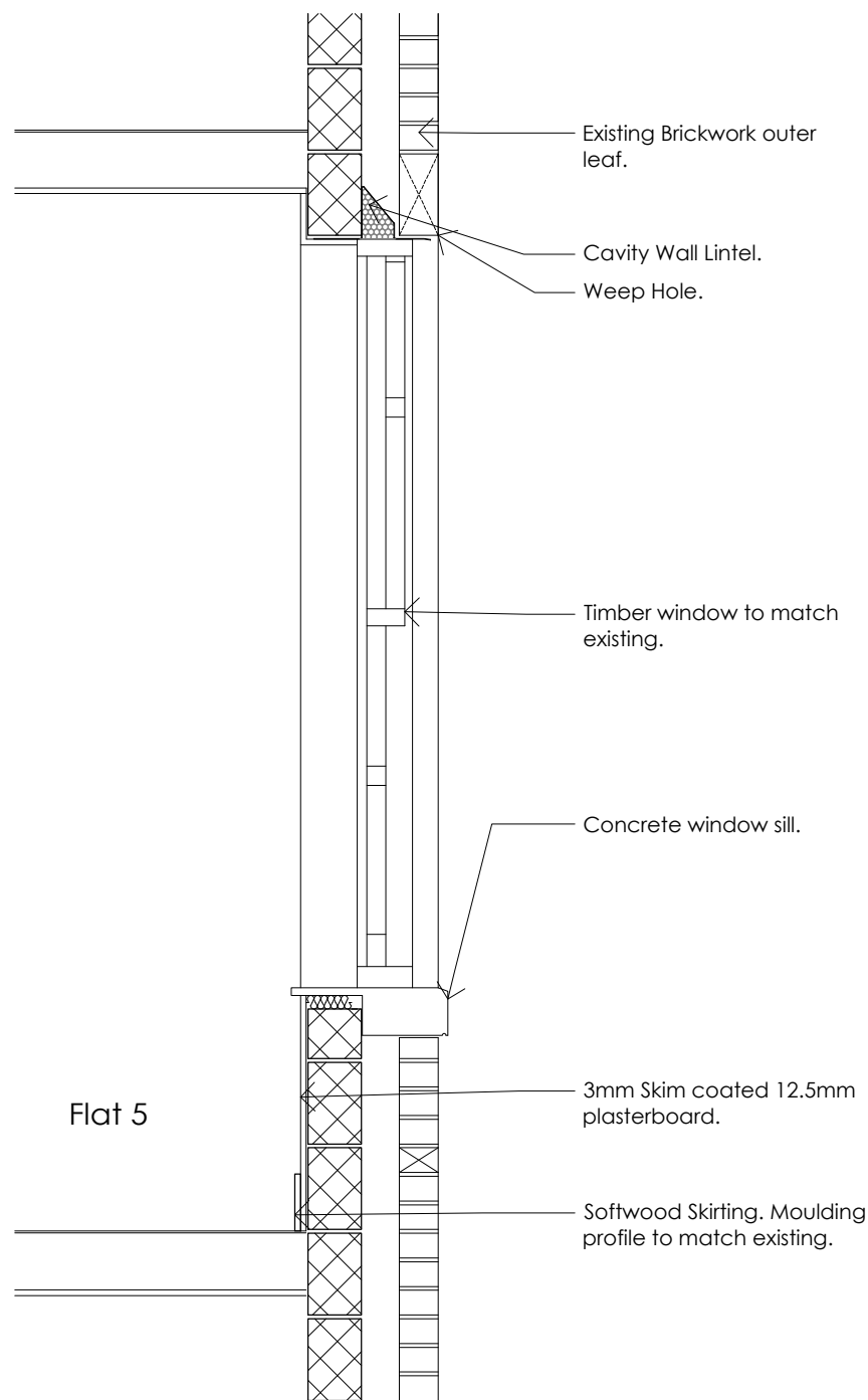
Window WS5 Detail 1:20
