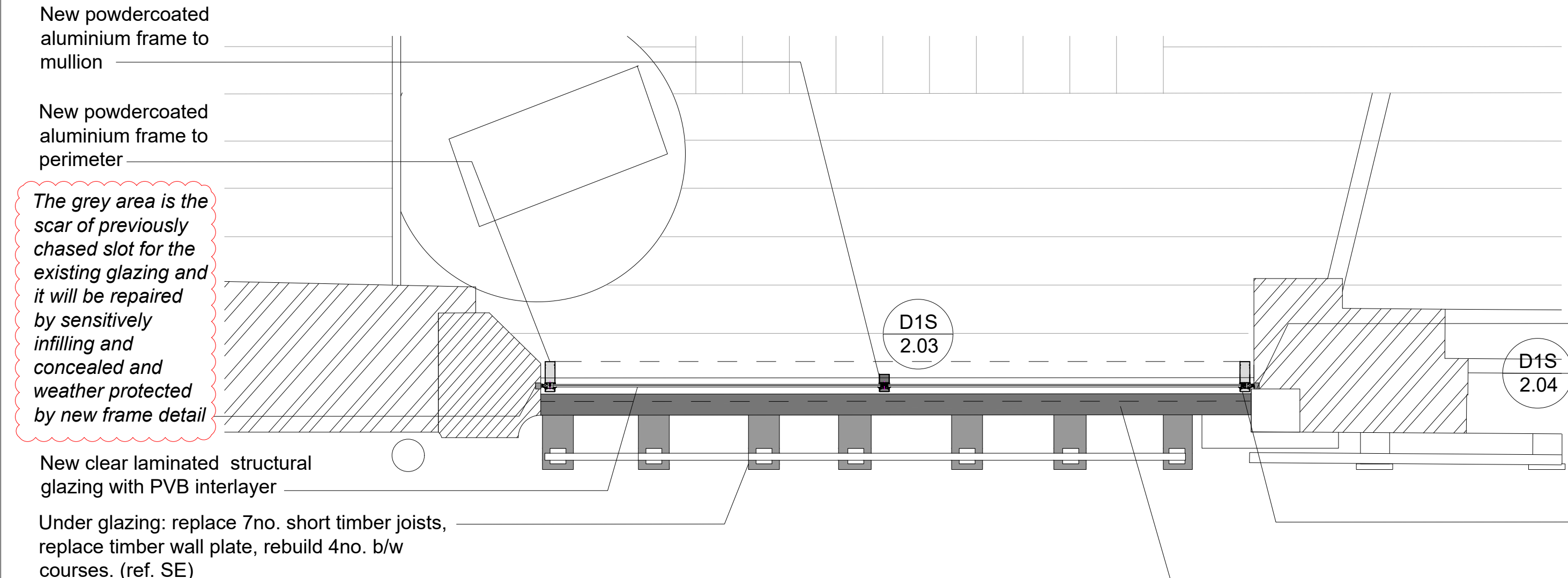
PLAN
