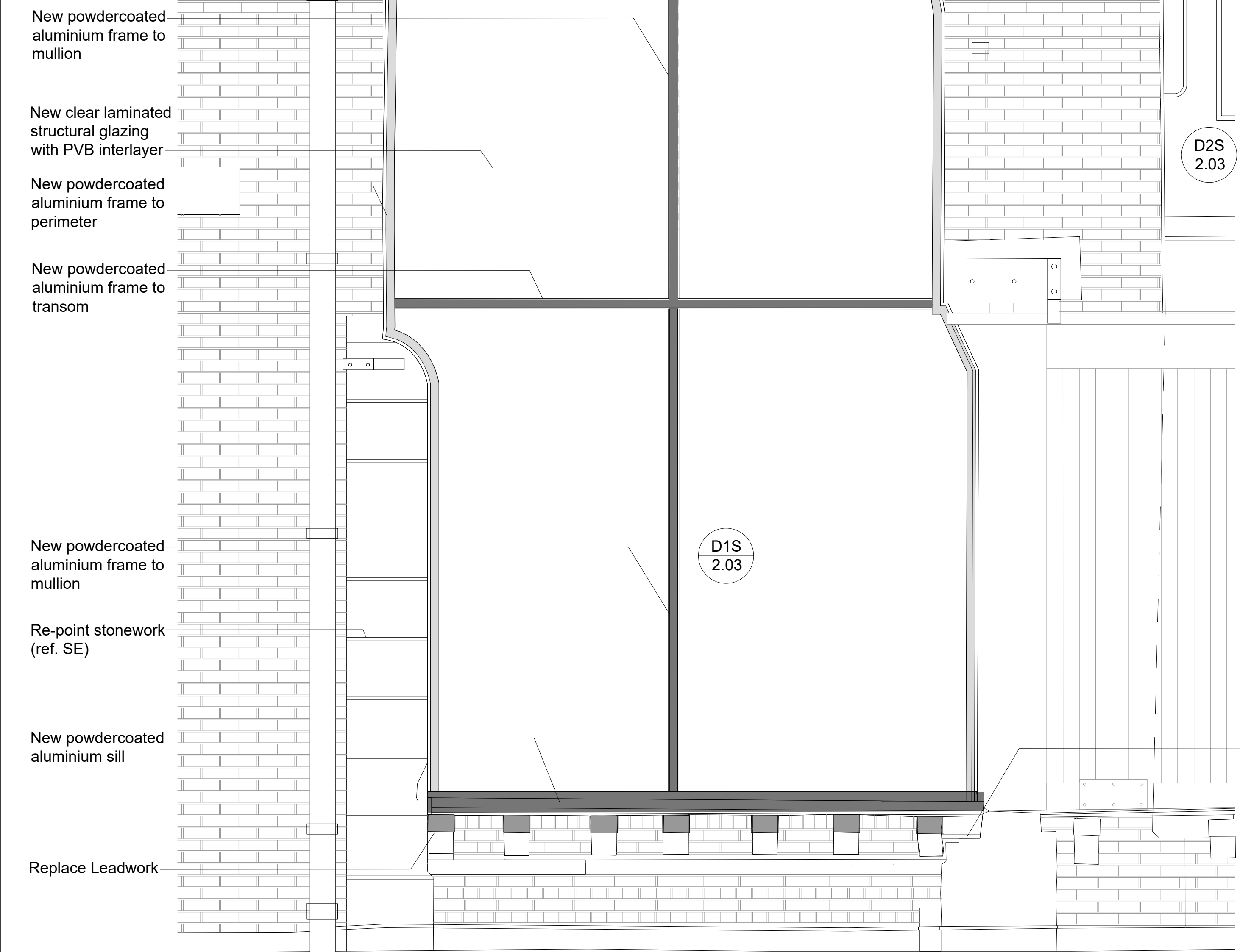
EXTERNAL ELEVATION
