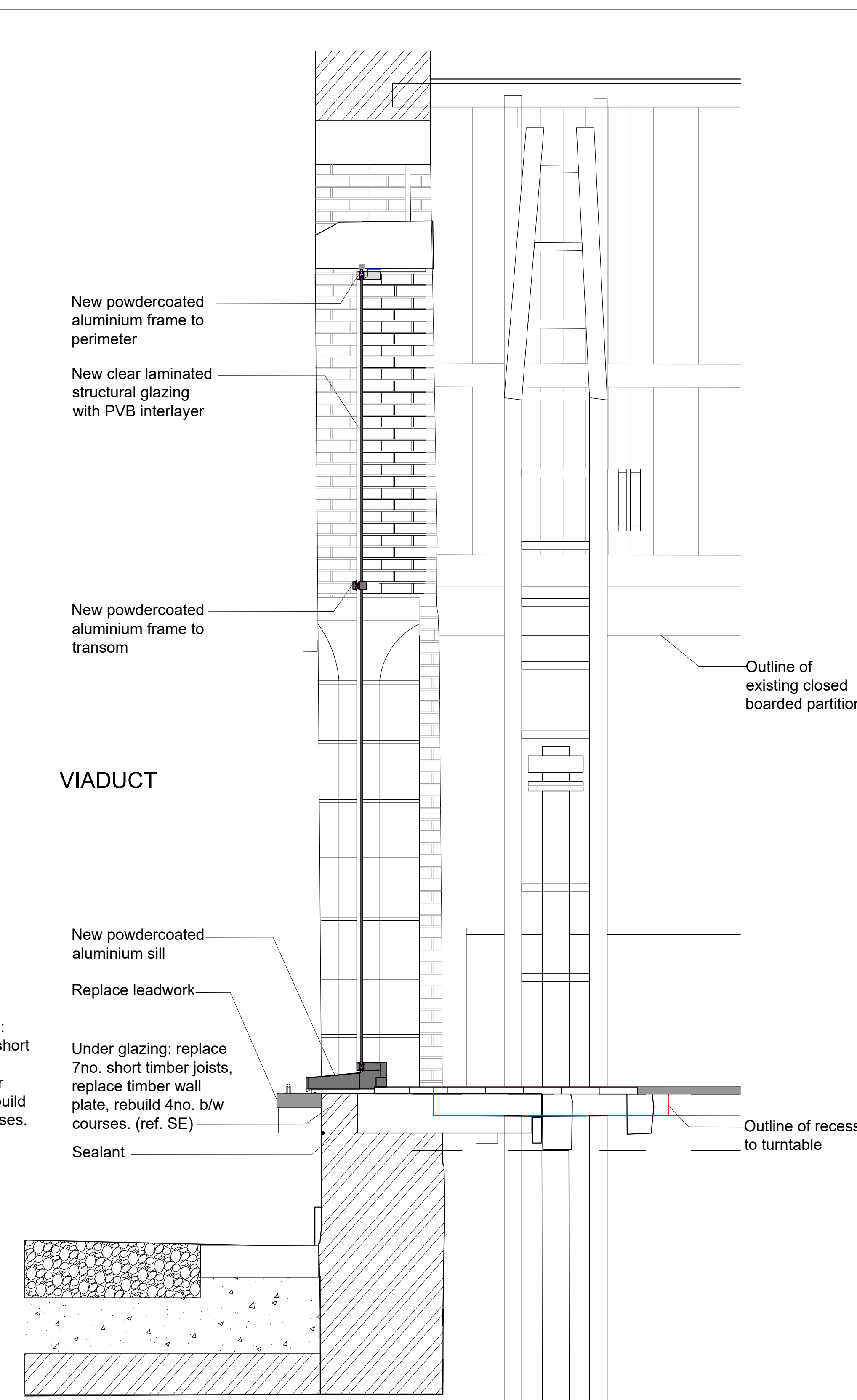
SECTION
