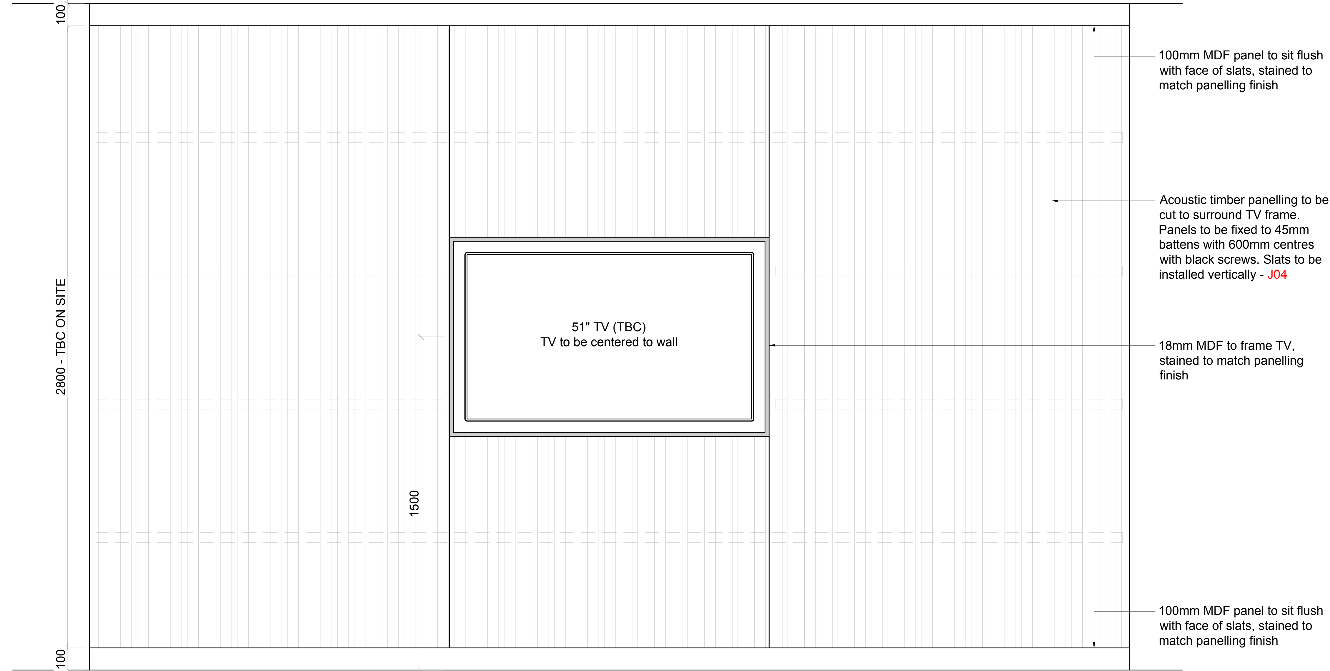
ELEVATION A 1:10 @ A1
