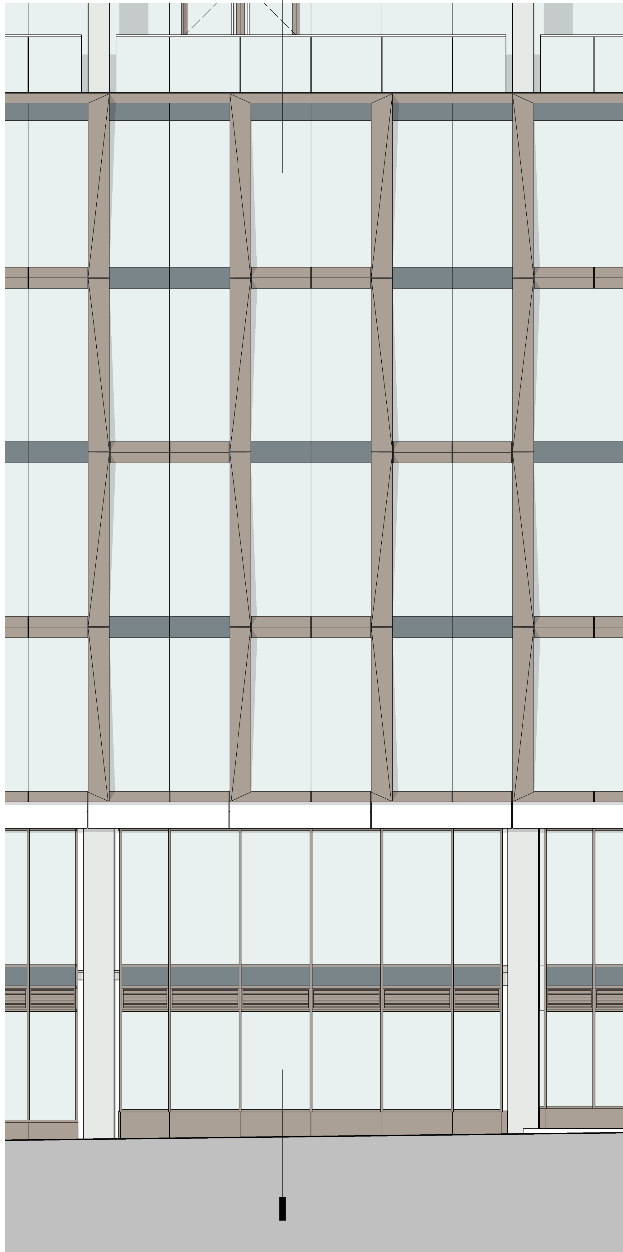
A7 TYP ENCLOSURE ELEVATION - OFFICE PODIUM 1 : 50
