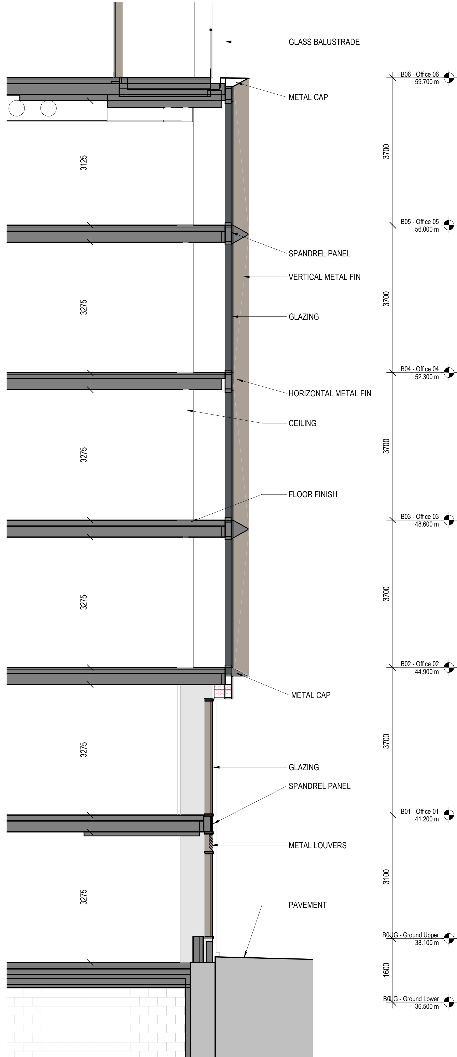
A3 TYP ENCLOSURE SECTION - OFFICE PODIUM 1 : 50
