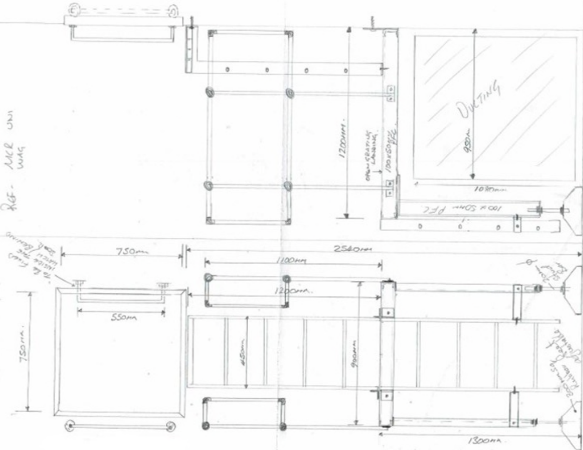
FRONT VIEW
