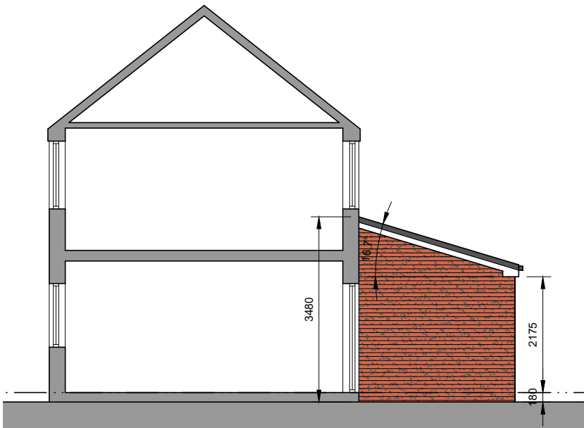
North West Facing Side Elevational Section
