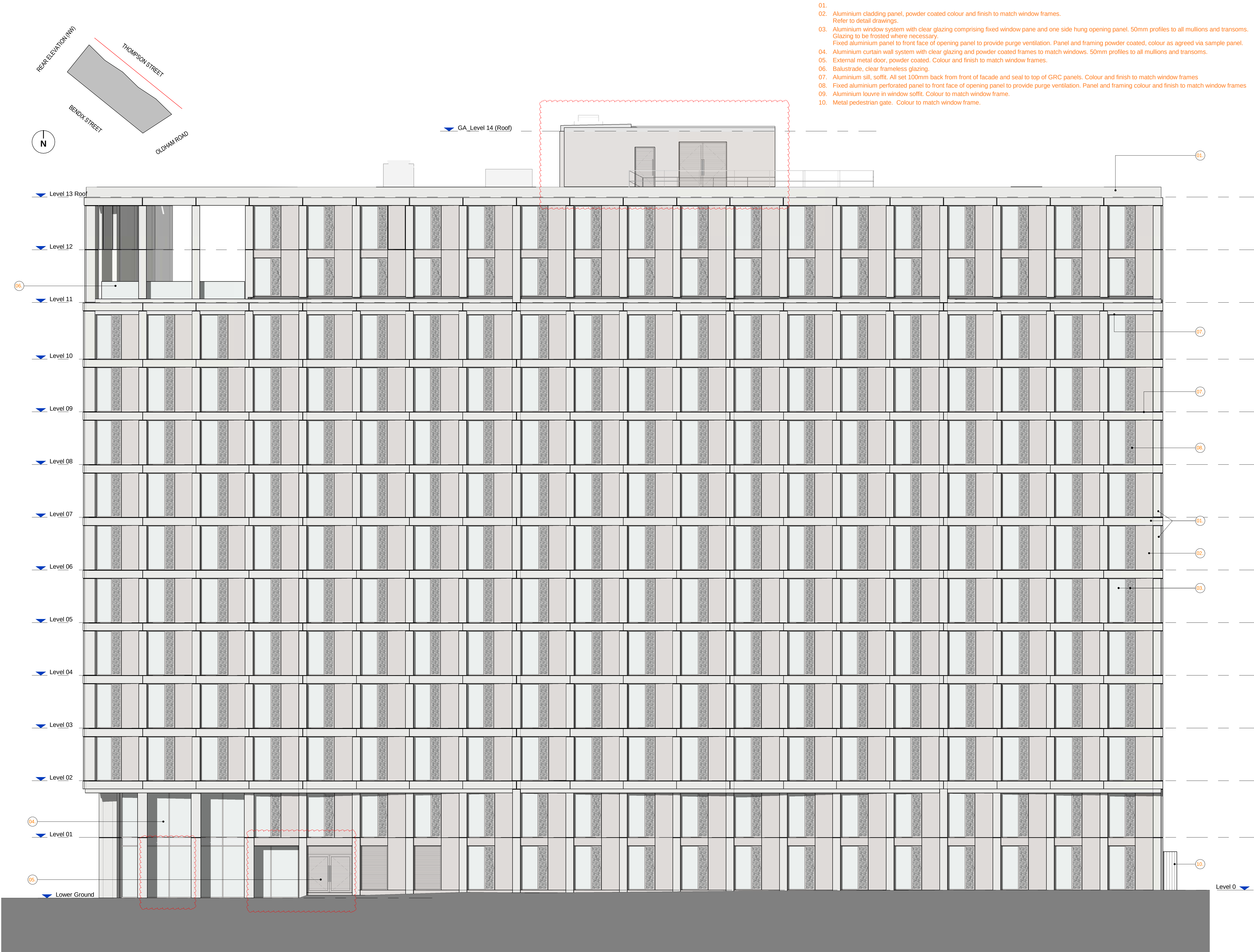
Thompson Street Elevation 1 : 100
