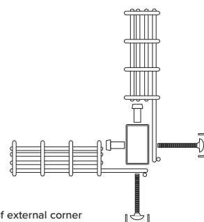
Plan of external corner
