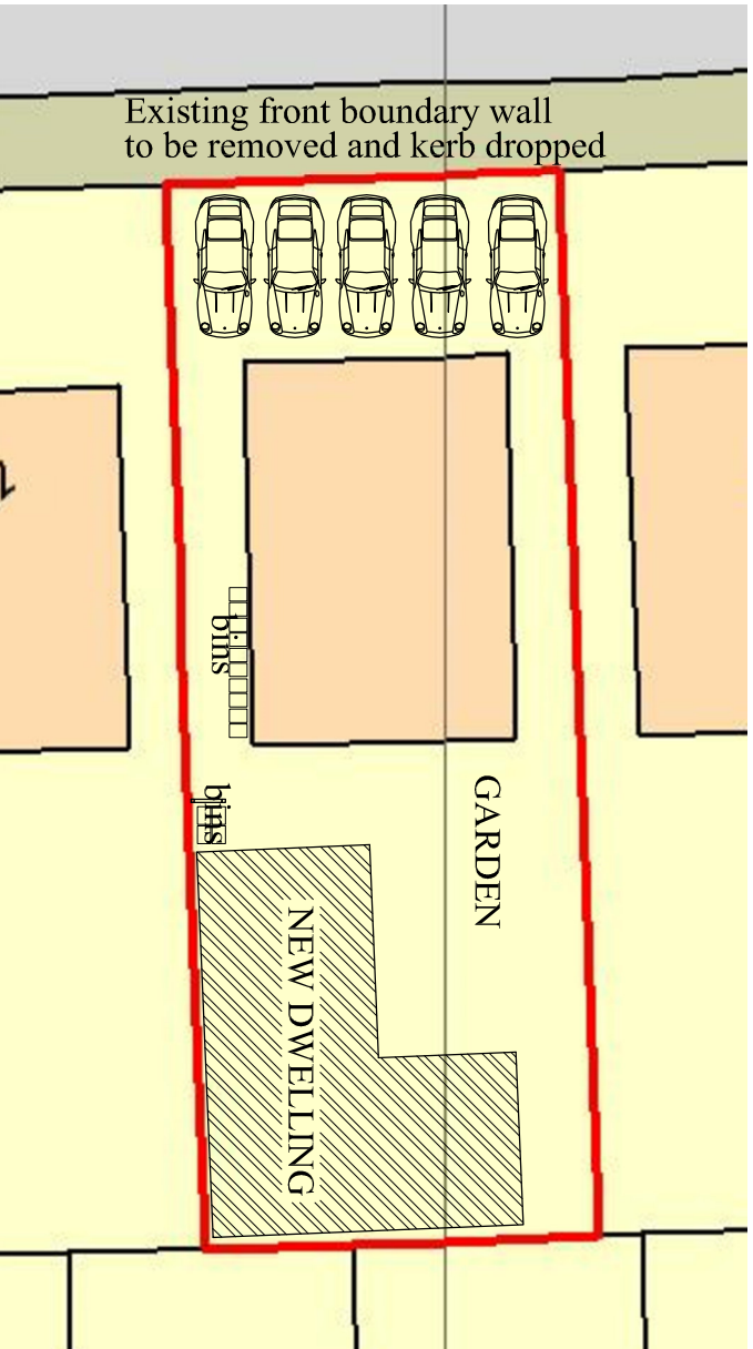
PROPOSED SITE PLAN 1:250
