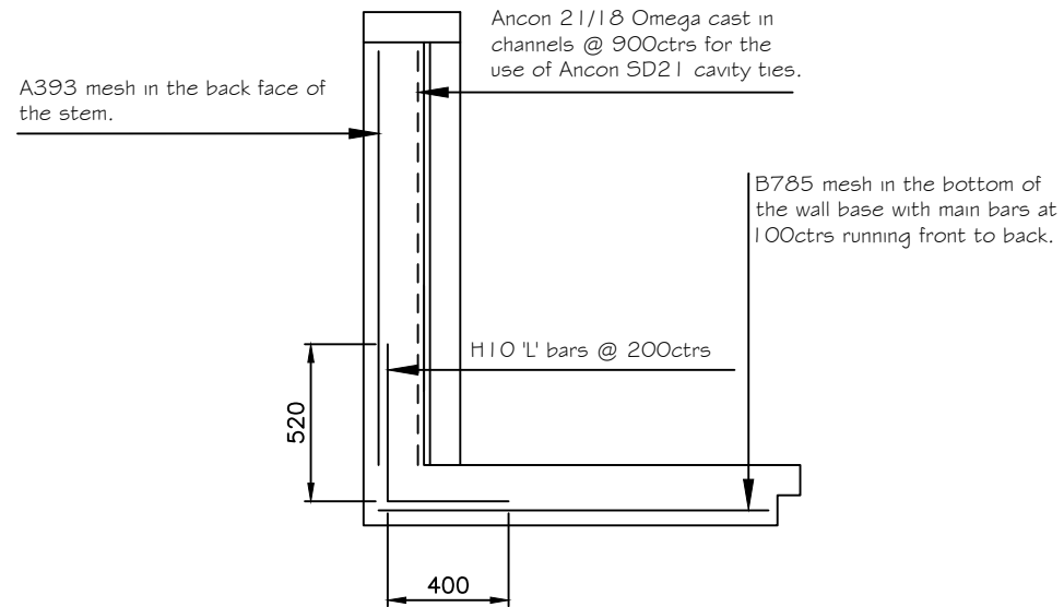
REBAR DETAILS AND WALL TIES (FRONT STAIRCASE) 1:20
