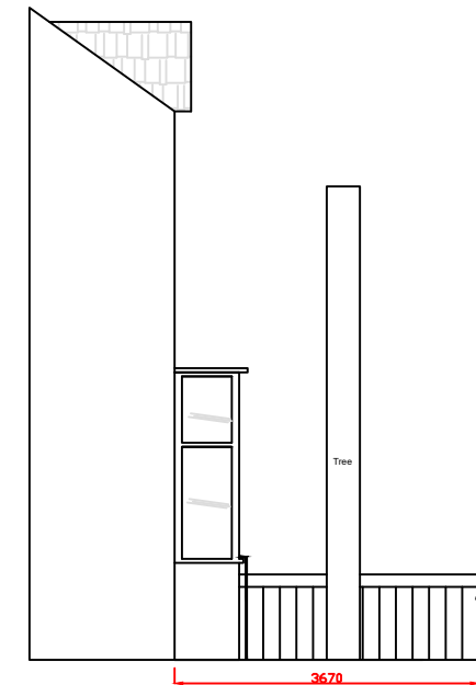
EXISTING LAYOUT view from 95
