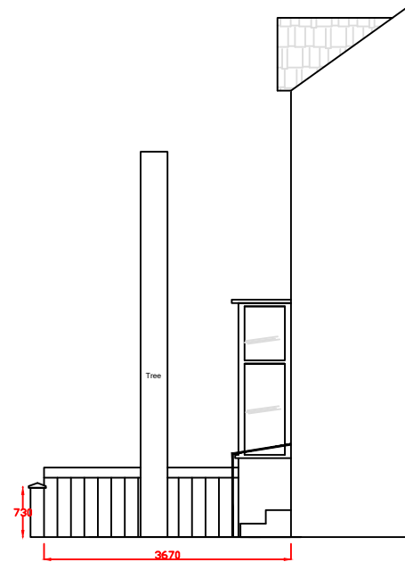
EXISTING LAYOUT view from 99
