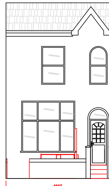
PROPOSED front LAYOUT
