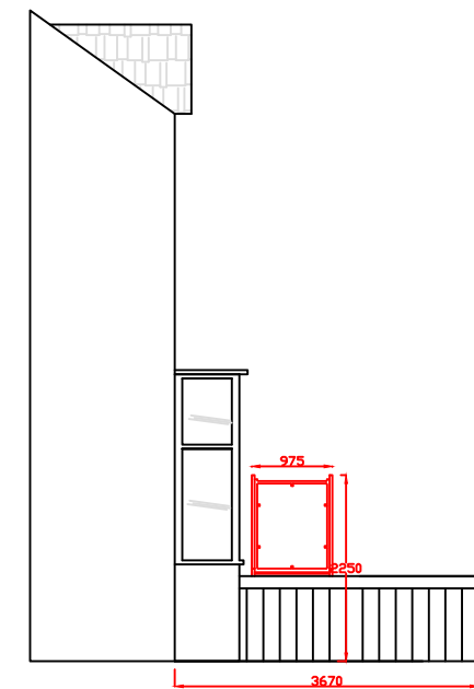
PROPOSED LAYOUT view from 95
