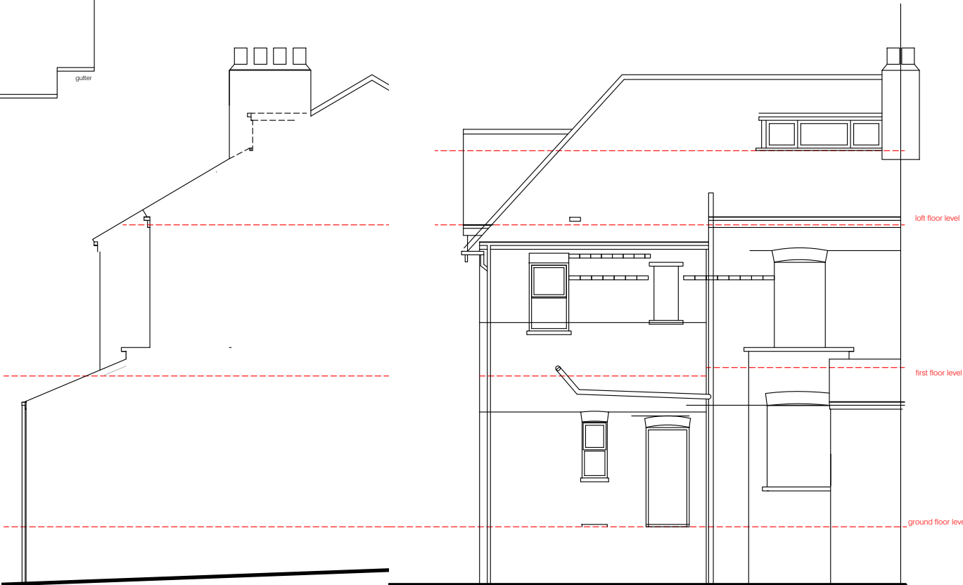
REAR ELEVATION AS EXISTING
