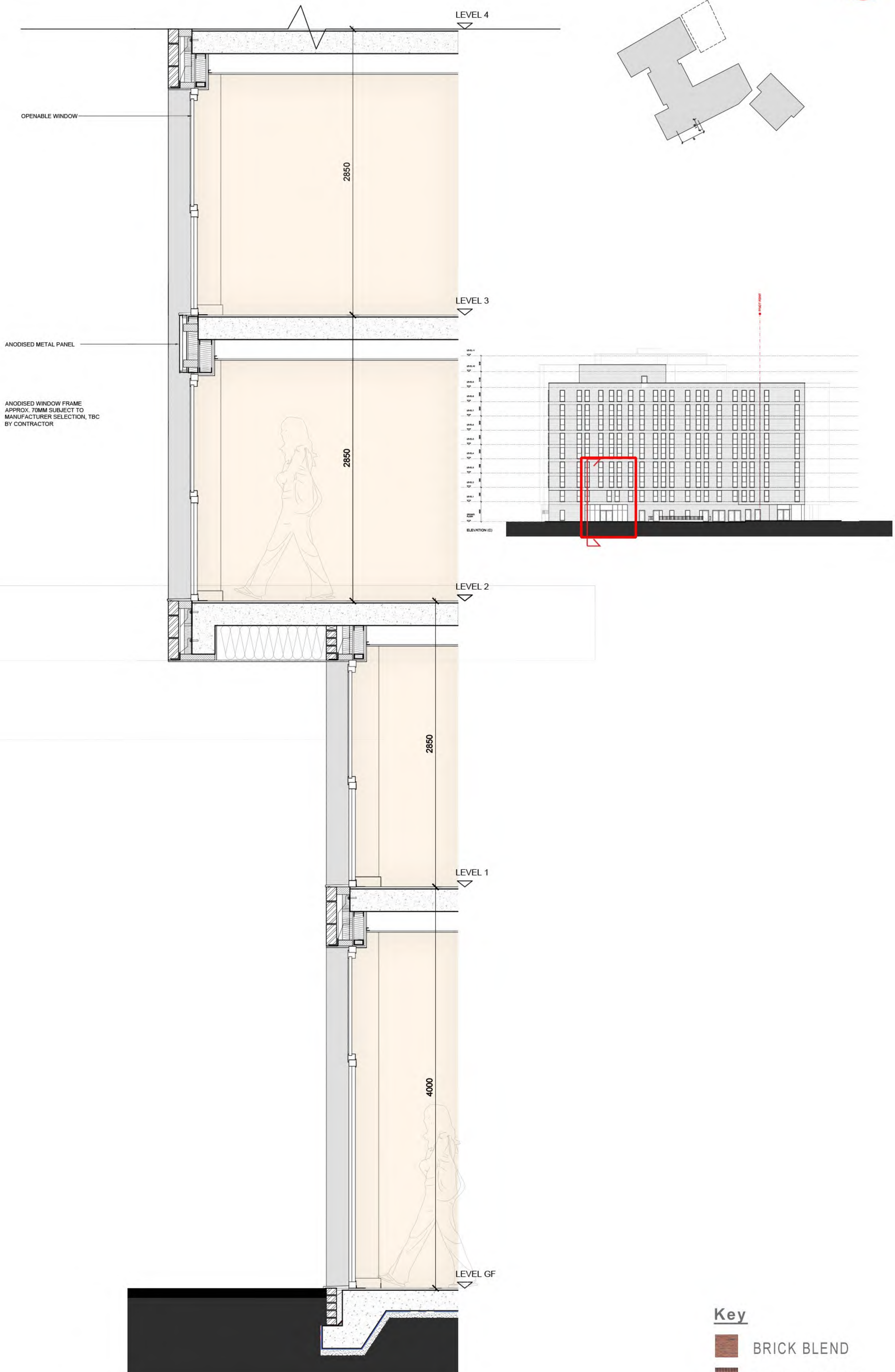
EXTERNAL WALL DETAIL SECTION B-1
