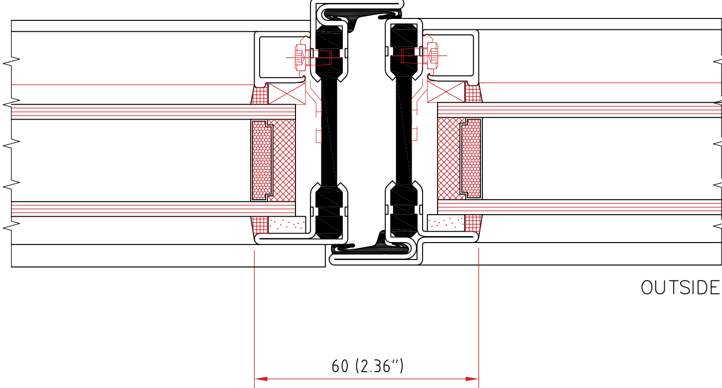
TYPICAL MEETING RAIL DETAIL (FRENCH CASEMENT)
