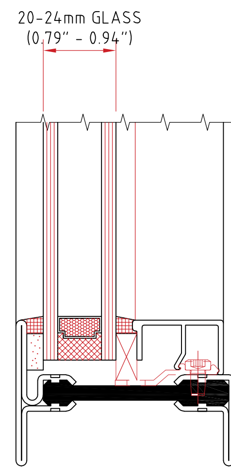
25mm (0.98") GLAZING BEAD
