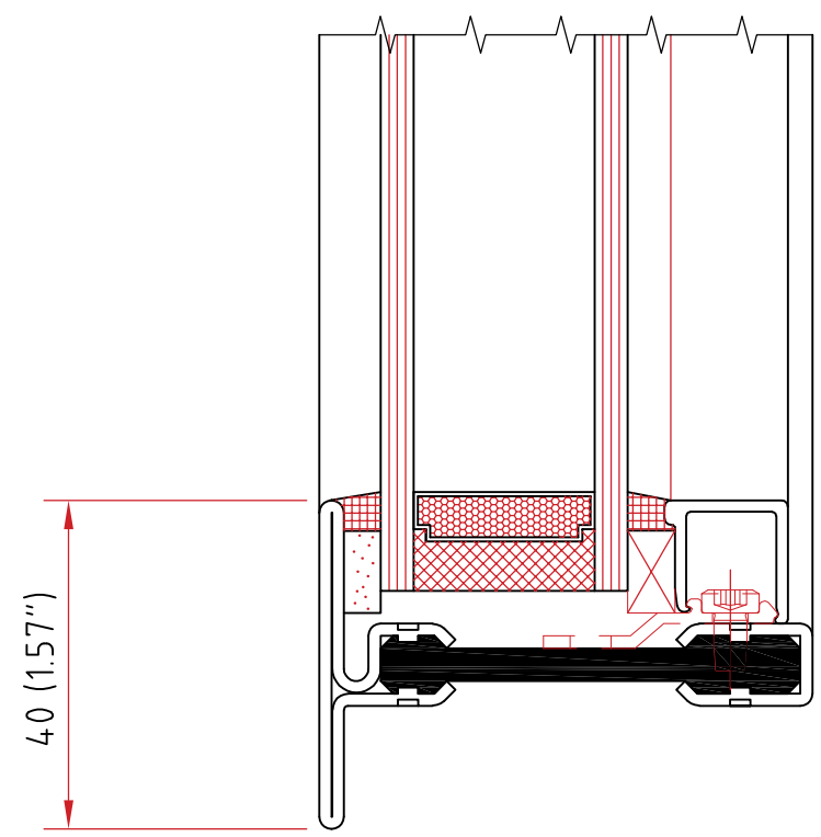
FIXED LIGHTS
