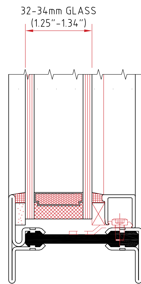
15mm (0.59") GLAZING BEAD
