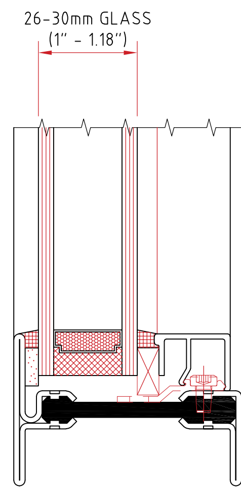
20mm (0.78") GLAZING BEAD
