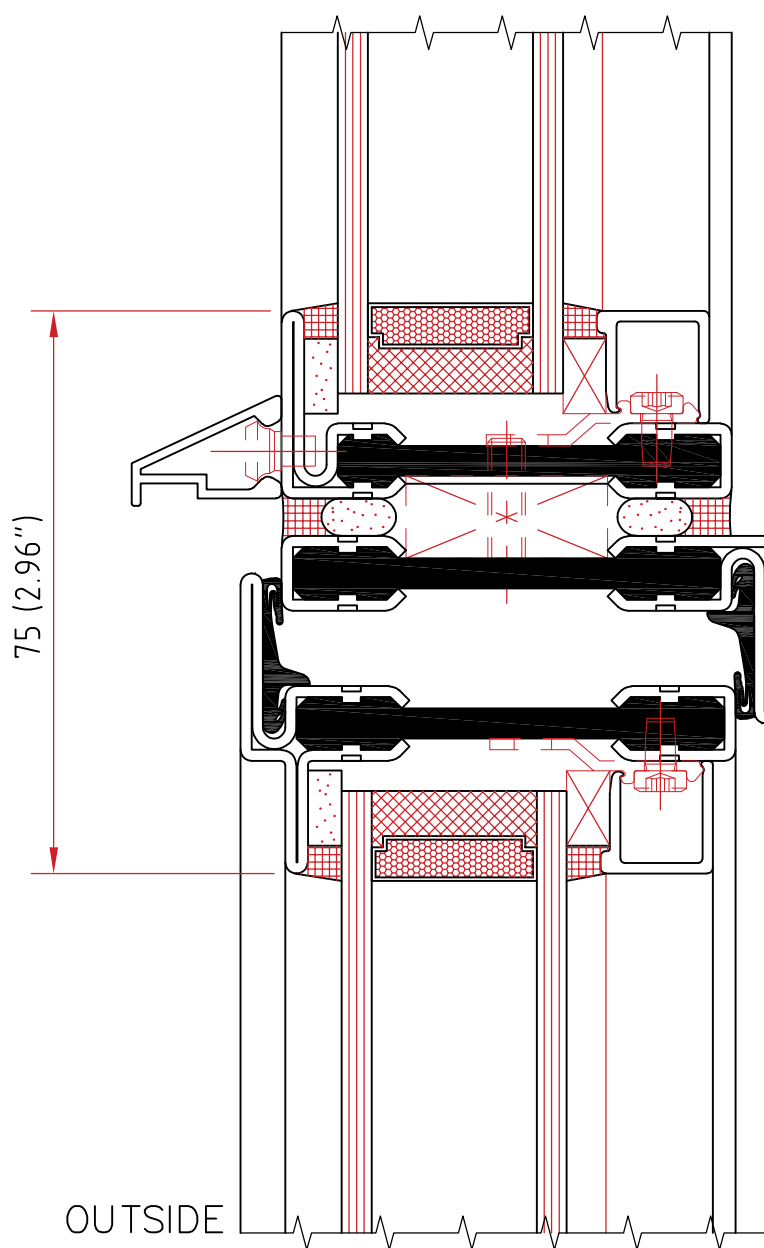
DIRECT COUPLING DETAILS
