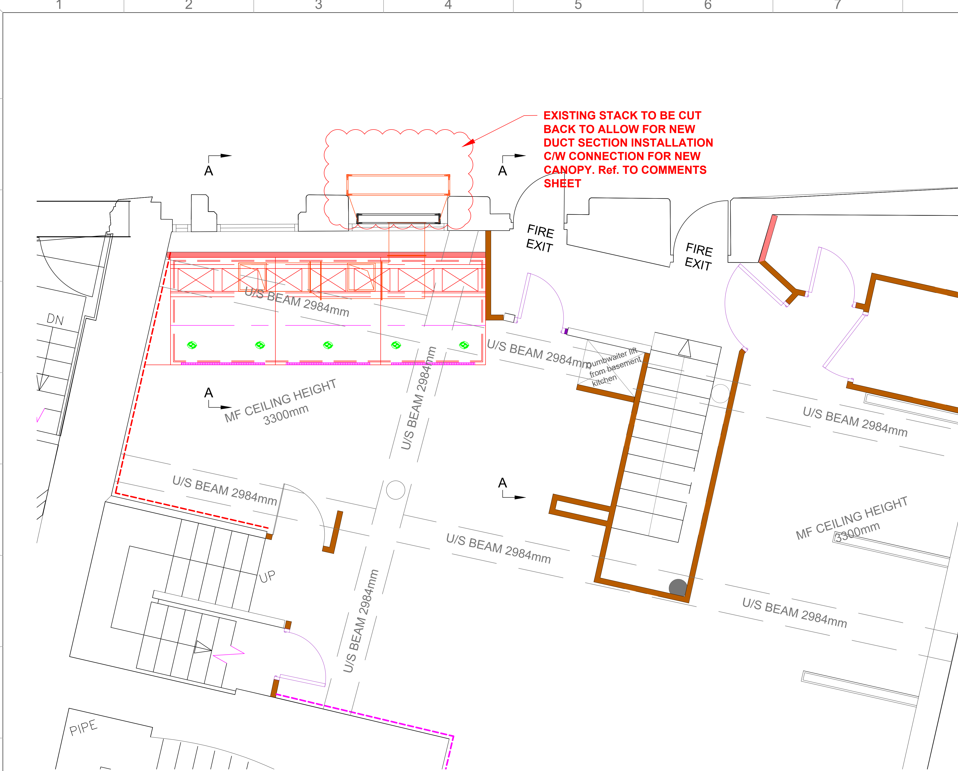
PLAN VIEW ON GROUND FLOOR CANOPY INSTALLATION
