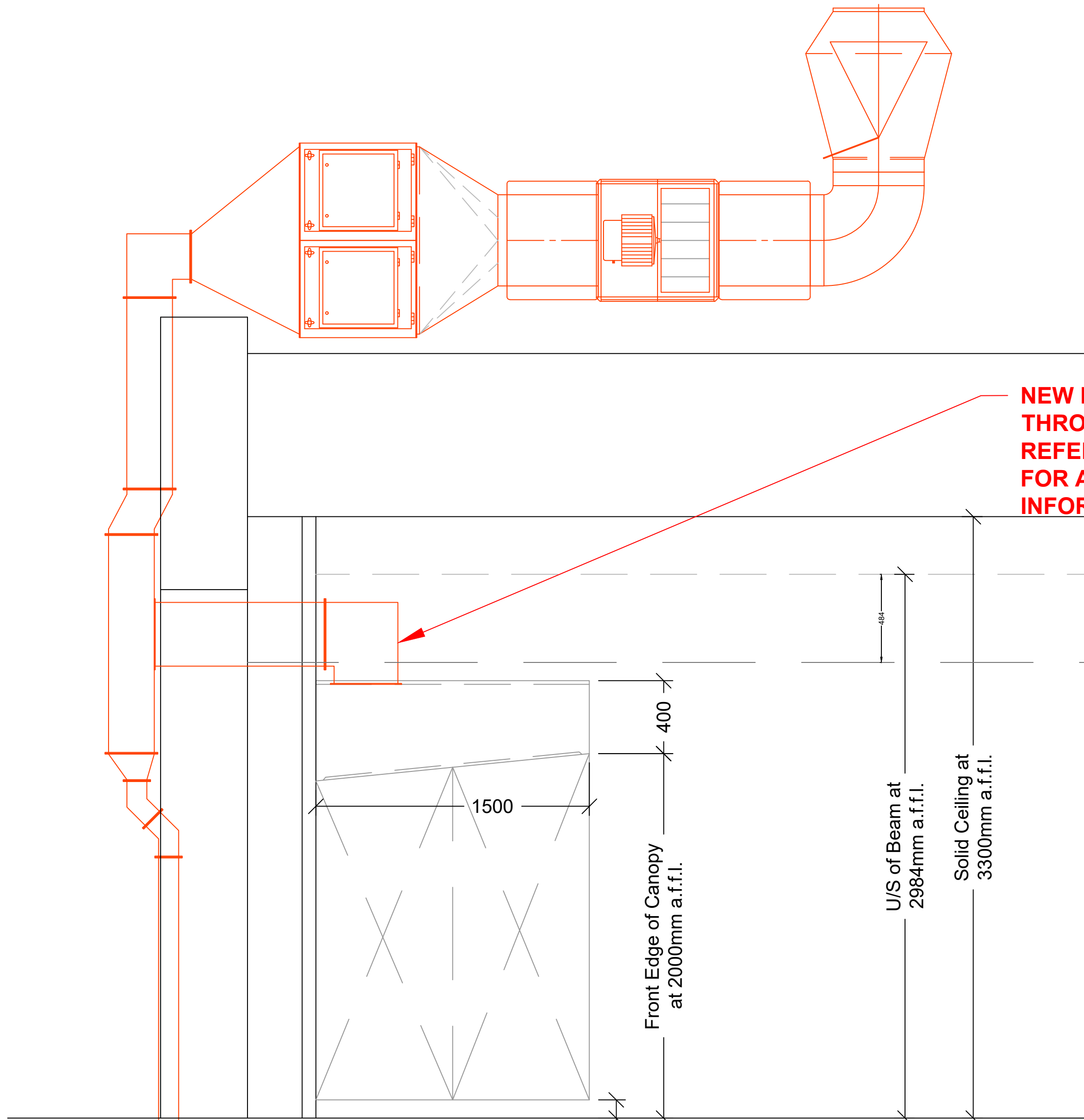
PROPOSED NEW CANOPY INSTALLATION ON ELEVATION A - A
