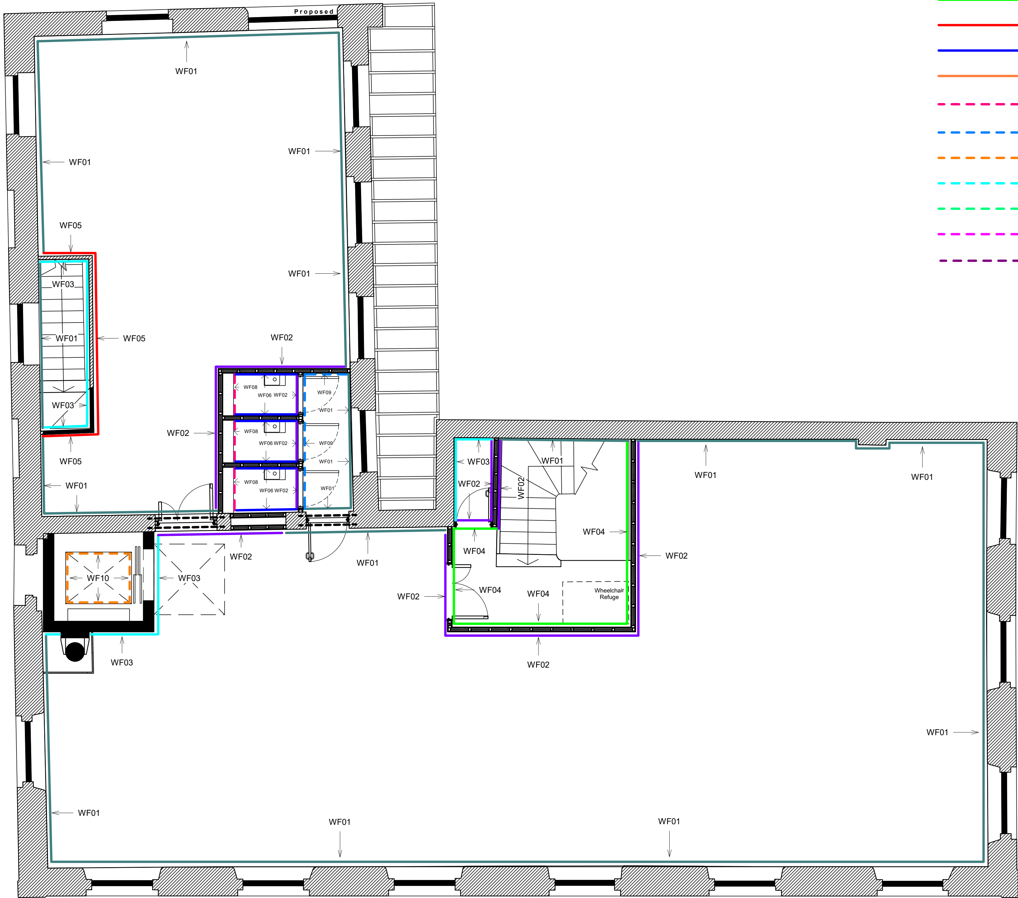
4FL Proposed Wall Finishes 1 : 50
