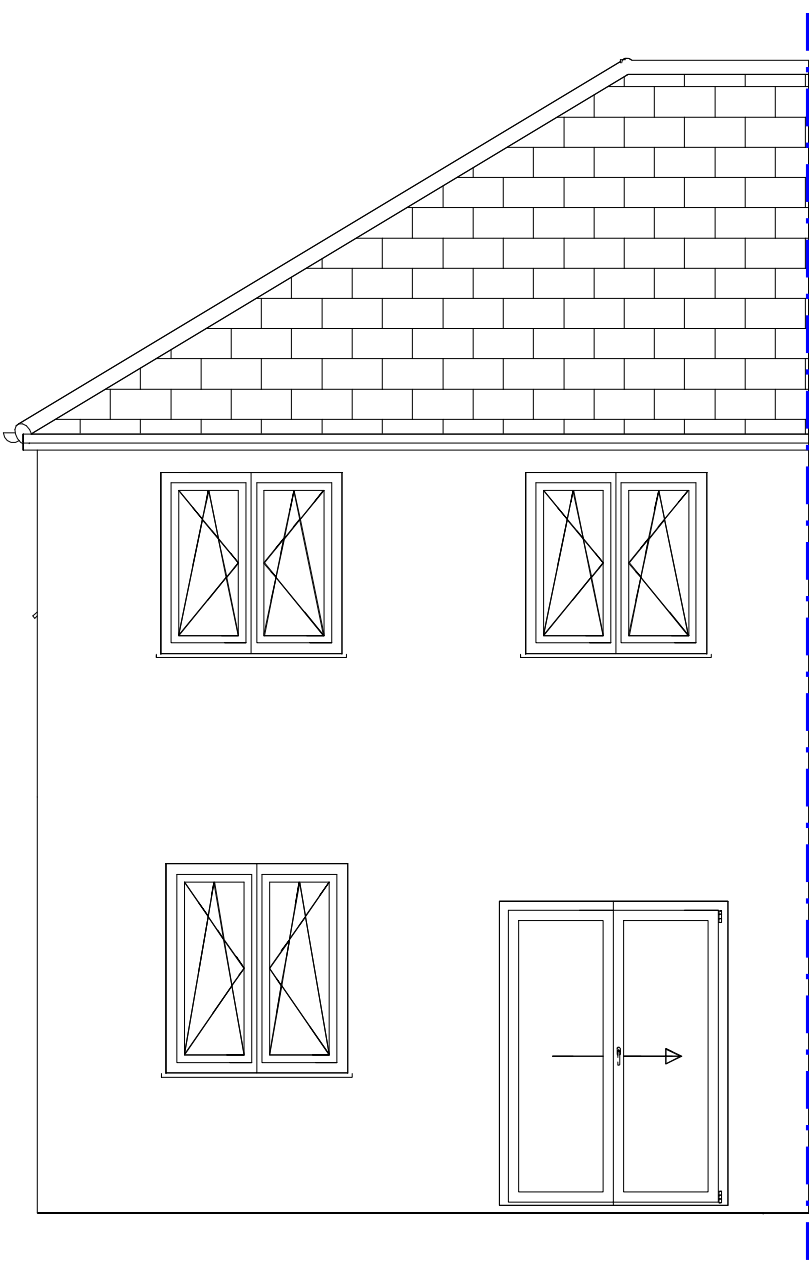
Existing North Elevation
