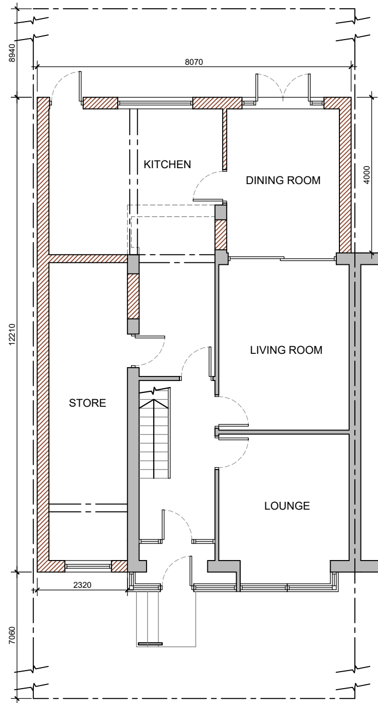
GROUND FLOOR 1:100
