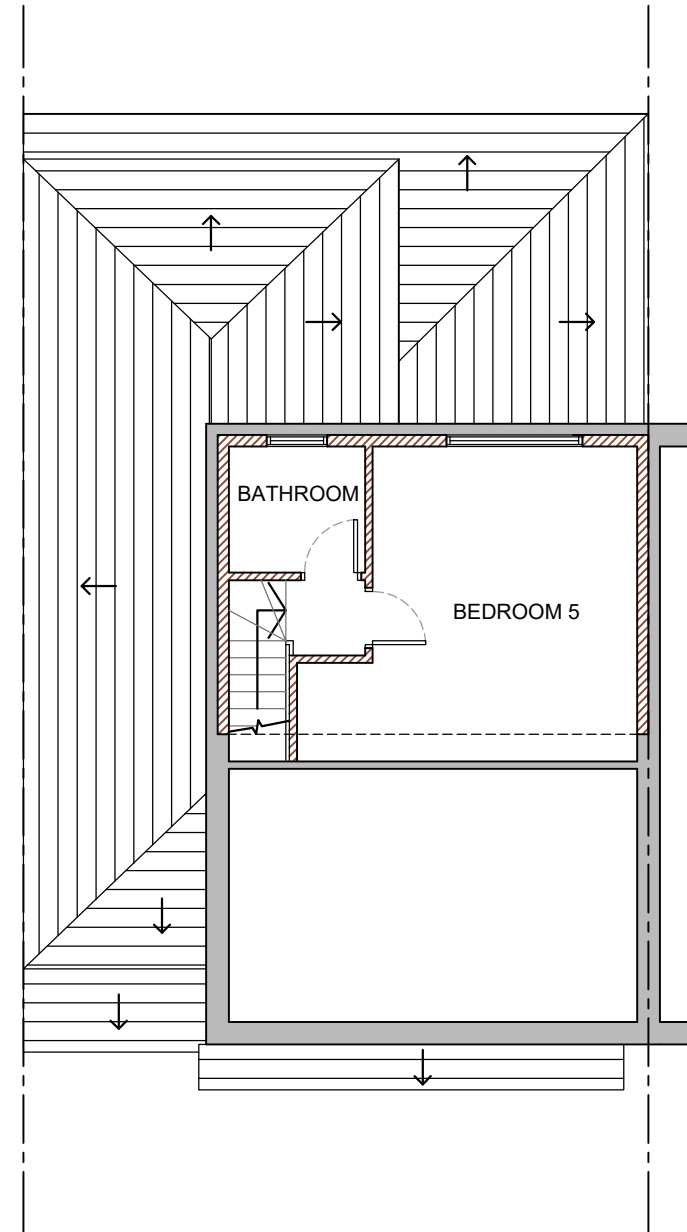
SECOND FLOOR 1:100
