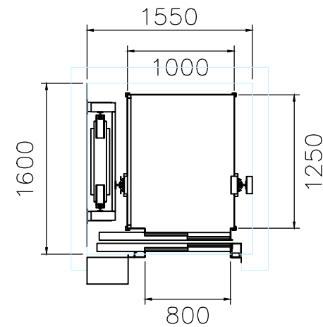
Stannah Core Xtralift MRL Traction Lift
