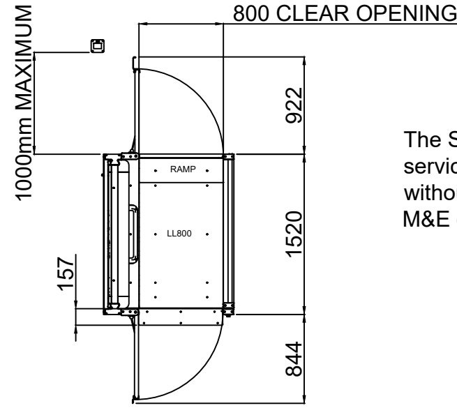
Stannah Lowrider LL800 Step Platform Lift
