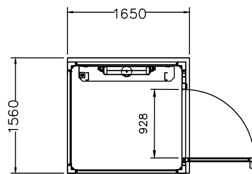
Stannah Midlift XL Plus Cabin Lift
