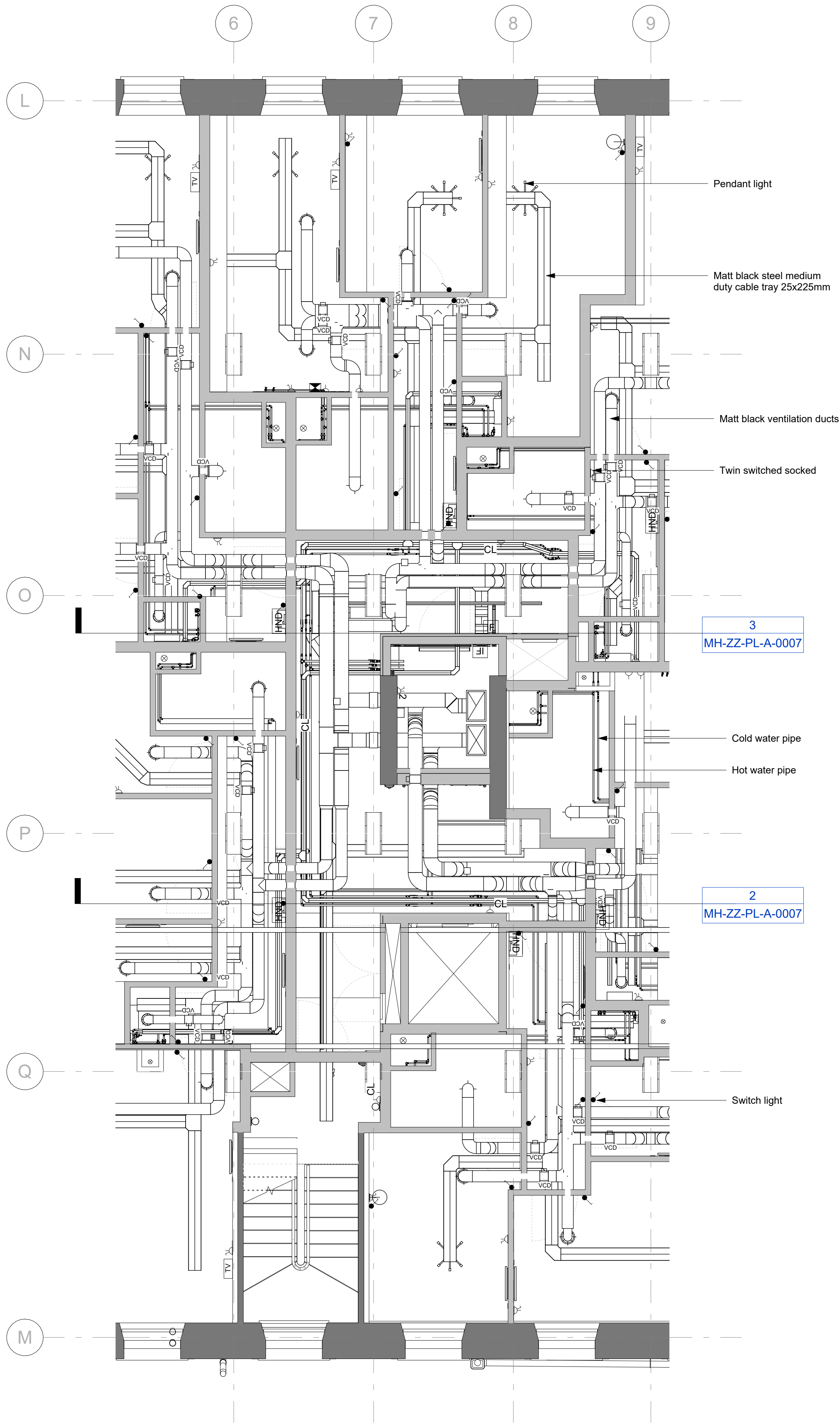
1 | MH-CORRIDOR SERVICES PLAN 1:50
