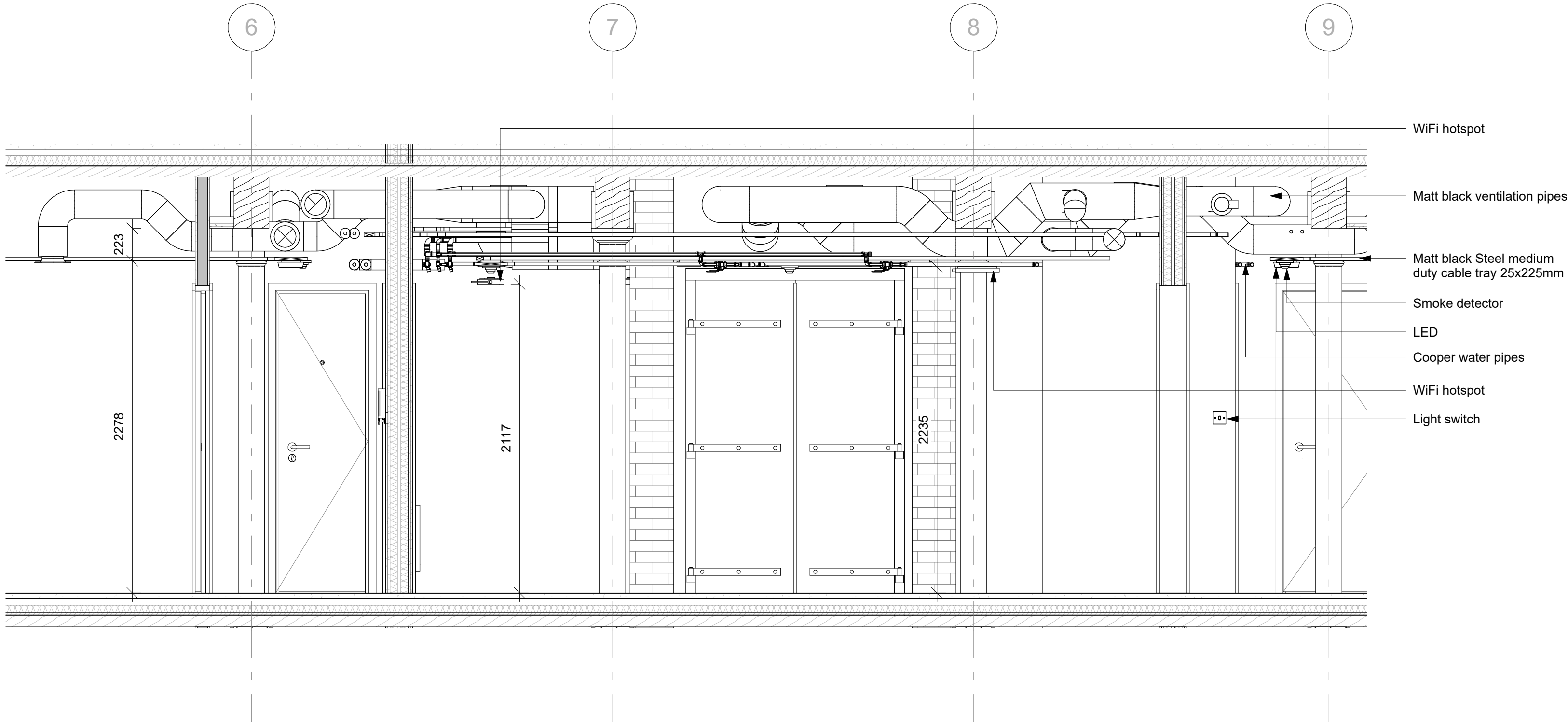
2 | CORRIDOR SECTION 1 1:25
