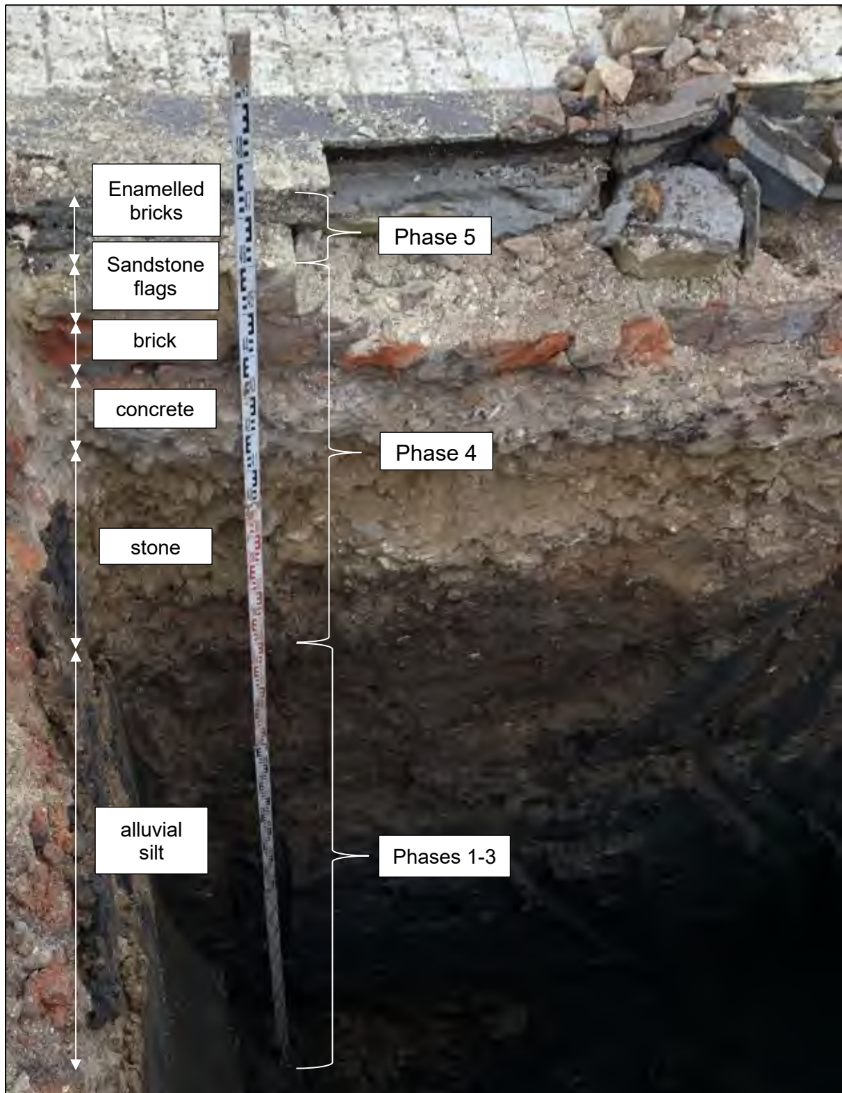
Plate_ : Sondage through the base of Pool 226 showing the composition of the foundations above earlier layers of alluvial silt
