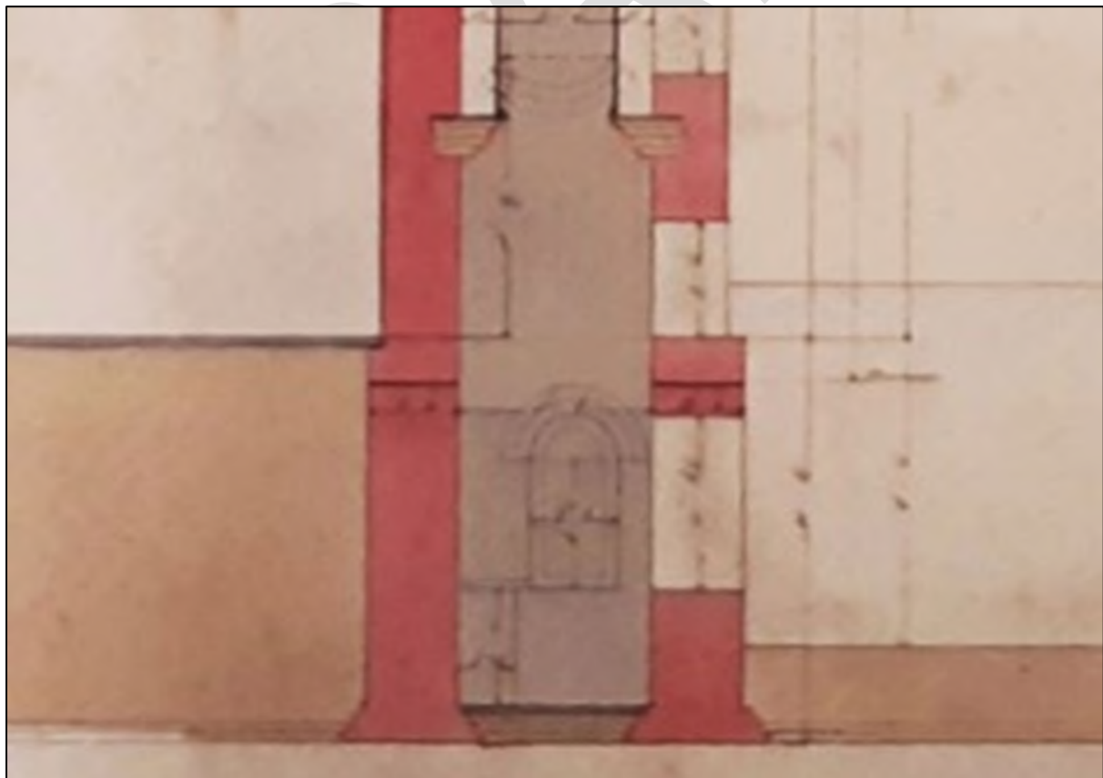
Plate x: Detail of chimney foundation illustrating the position of the flues
