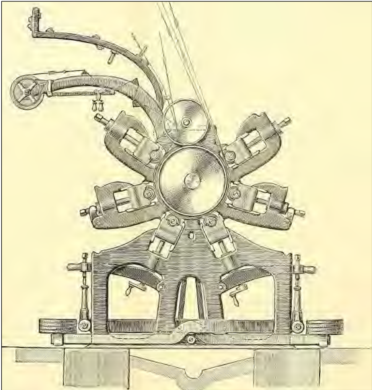
Plate xx: A six colour printing machine depicted in 'The Printing of Cotton Fabrics' (Sansone 1887)
