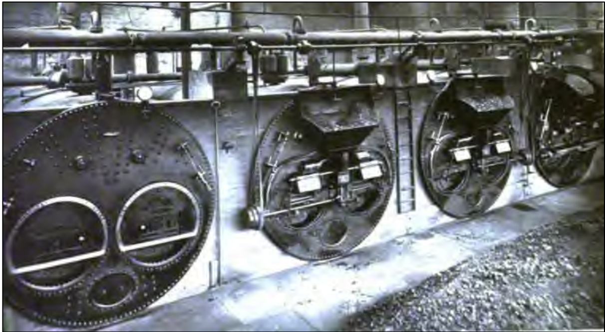
Plate x: An example of a bank of Lancashire boilers, some fitted with automatic feeders (hoppers)
