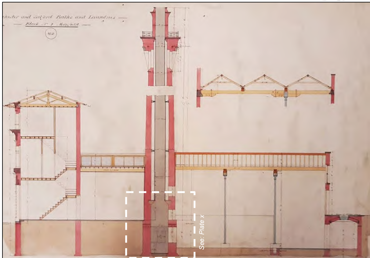
Plate xx: Cross-section through the northern part of Mayfield Baths with detail of chimney foundation
