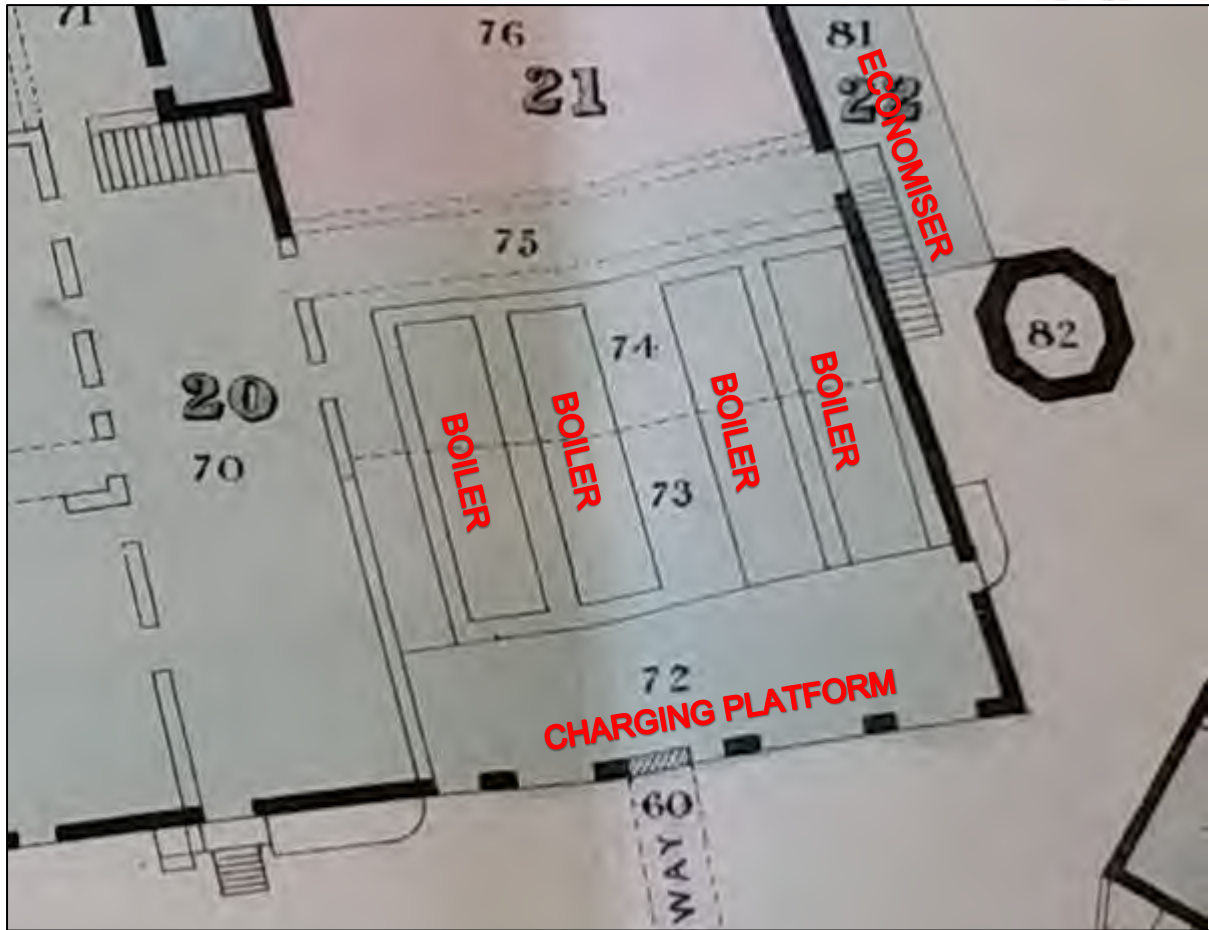
Plate xx: Extract from the 1872 insurance plan showing the internal layout of the boiler house
