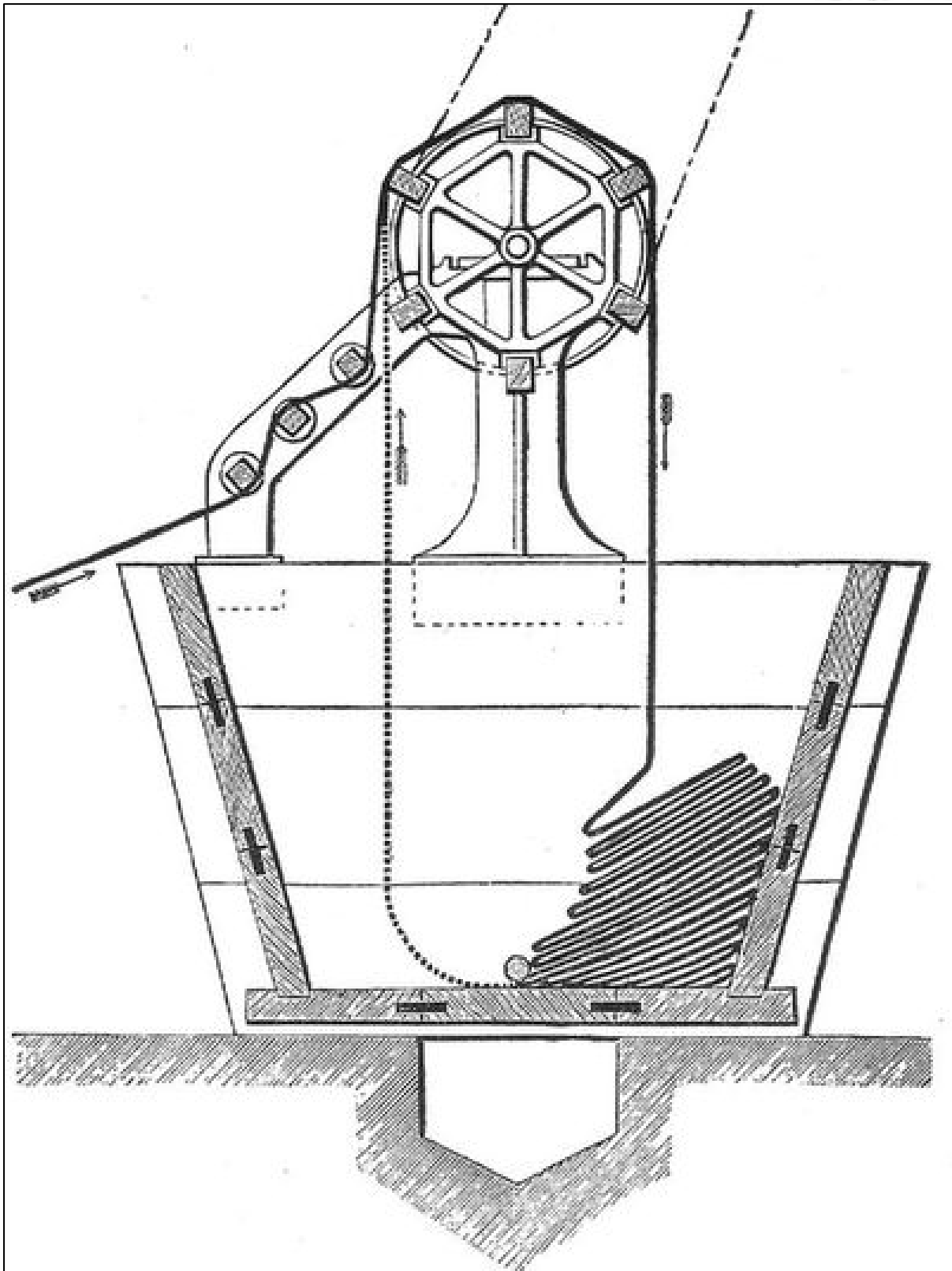
Plate x: Diagram of a wince dye beck or dye digger
