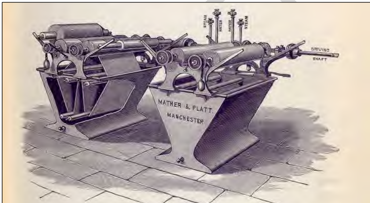
Plate x: Dye jigger
