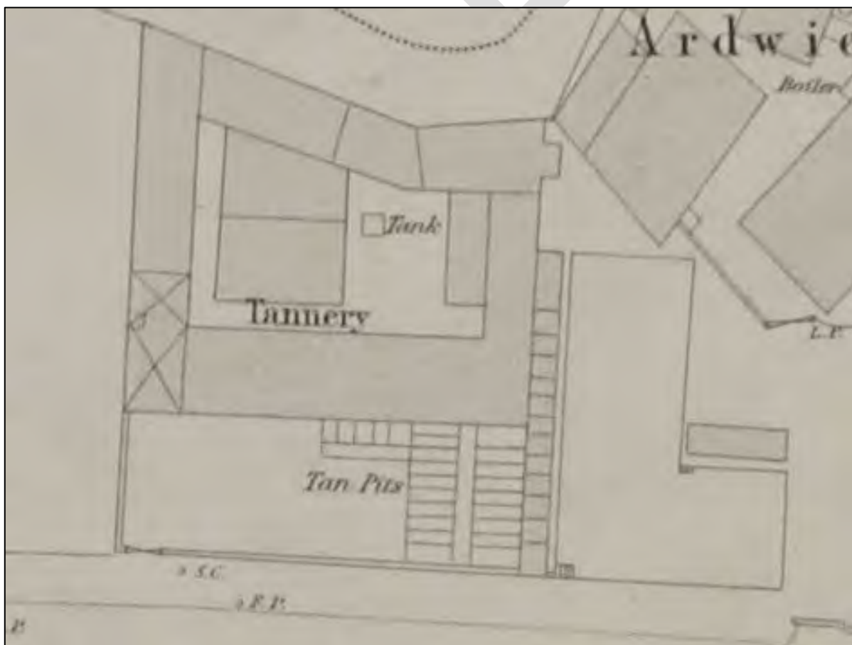
Plate xx: Extract from the 1851 Town Plan map showing the layout of the Ardwick Tannery.
