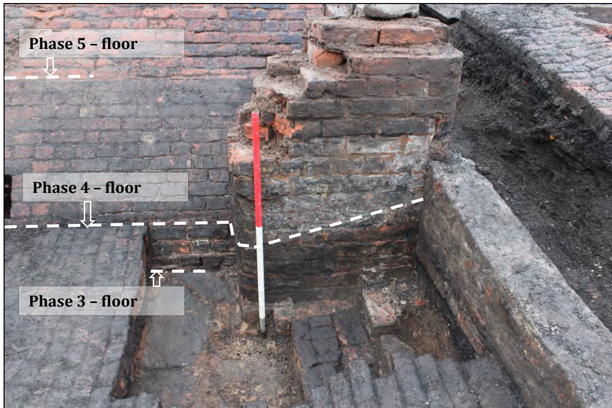
Plate_ : The three successive charging floors revealed within the southern half of the boiler house: 3172 ( Phase 3 ); 3065 ( Phase 4 ) and 3174 ( Phase 5 ). Photographed looking south (1m scale)
