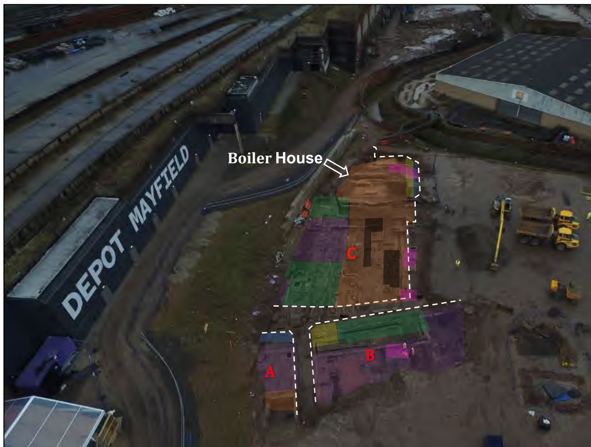
Plate 1: Oblique aerial view across the excavation of Mayfield Dye Works, looking east, showing the excavated portions of Buildings A, B and C and their main phases of development. Seven building phases were identified, each is colour-coded: 1 – purple; 2 – green; 3 – orange; 4 – yellow; 5 – blue; 6 – grey; 7 – pink. The River Medlock is visible in the rear of the shot.
