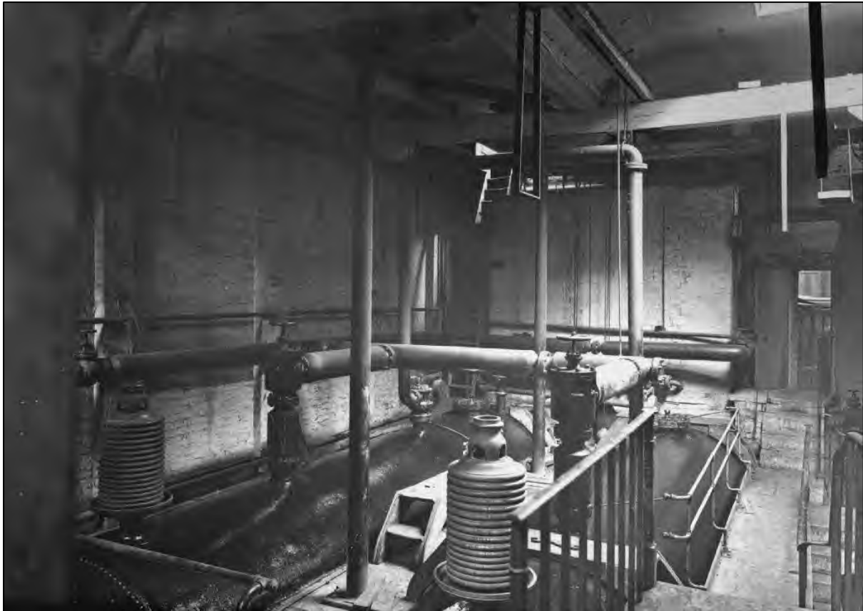
Plate x: Photograph showing the two steam boilers at Mayfield Baths
