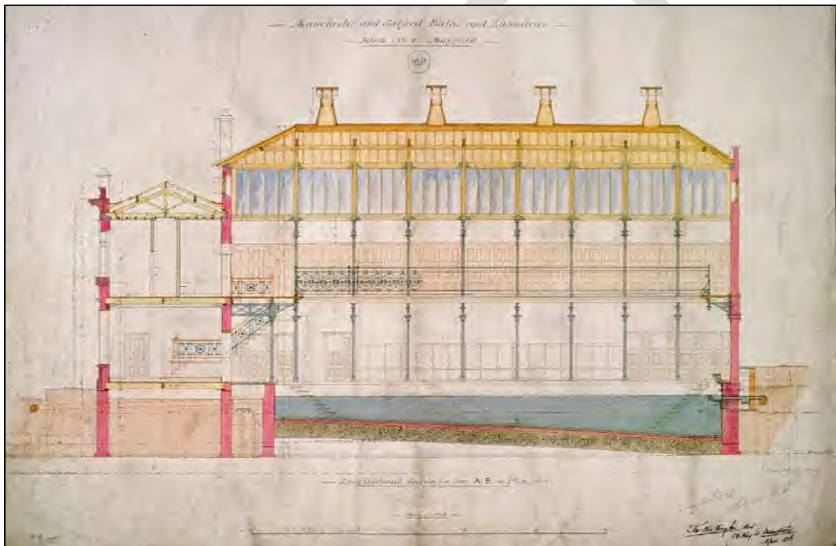
Plate x: Worthington's design plan of Mayfield Baths, drawn on canvas by Thomas Worthington in April 1856
