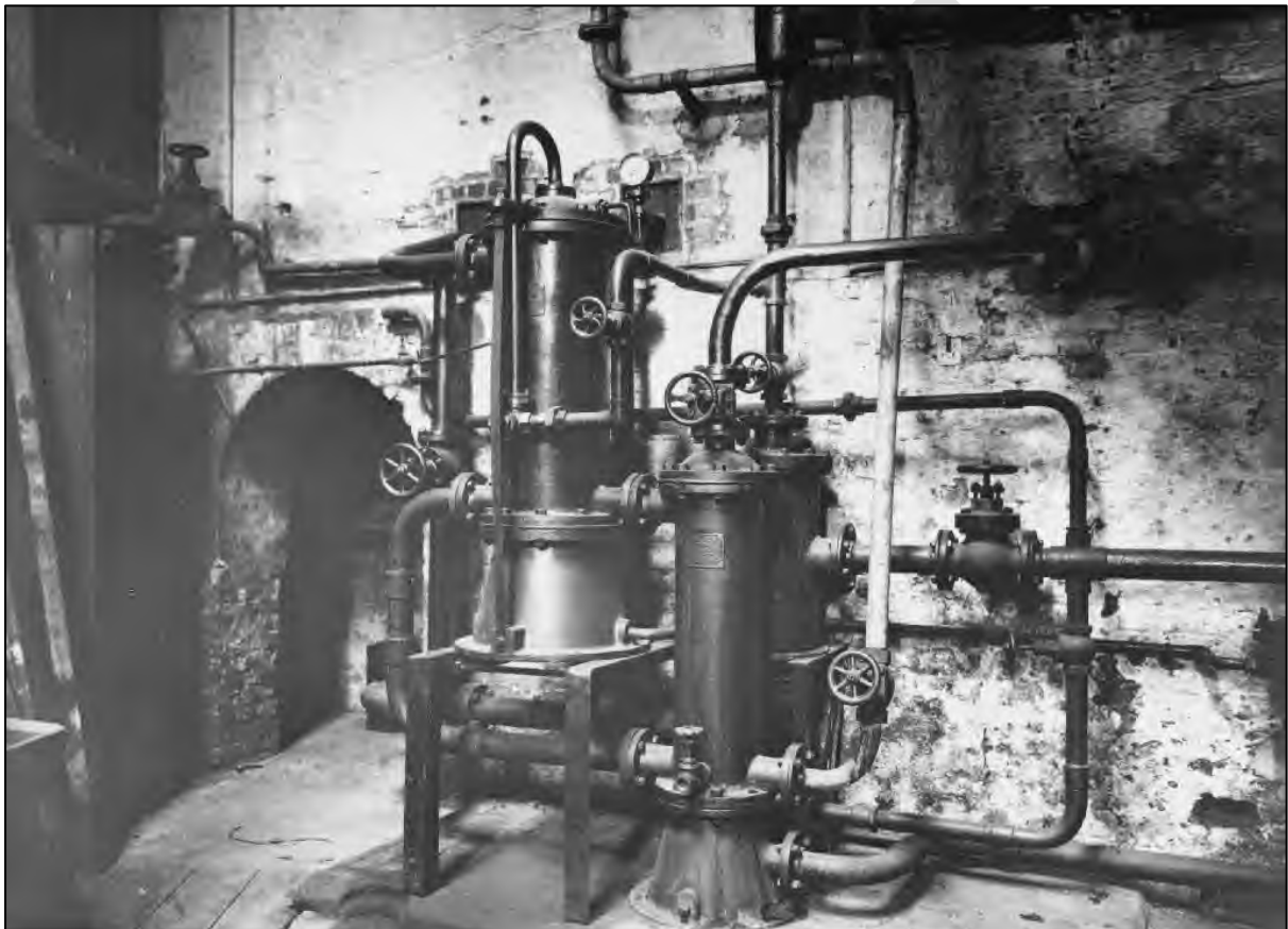
Plate xx: The Royle Calorifier at Mayfield Baths, 1902.
