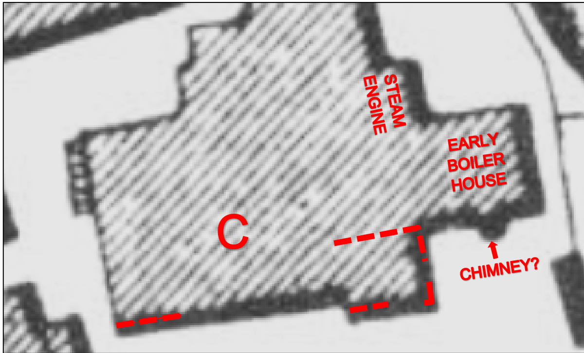
Plate x: Extract from Bancks and Co's 1831 map showing the Phase 2 walls revealed in Area 3, Building C, together with the location of the early engine and boiler houses
